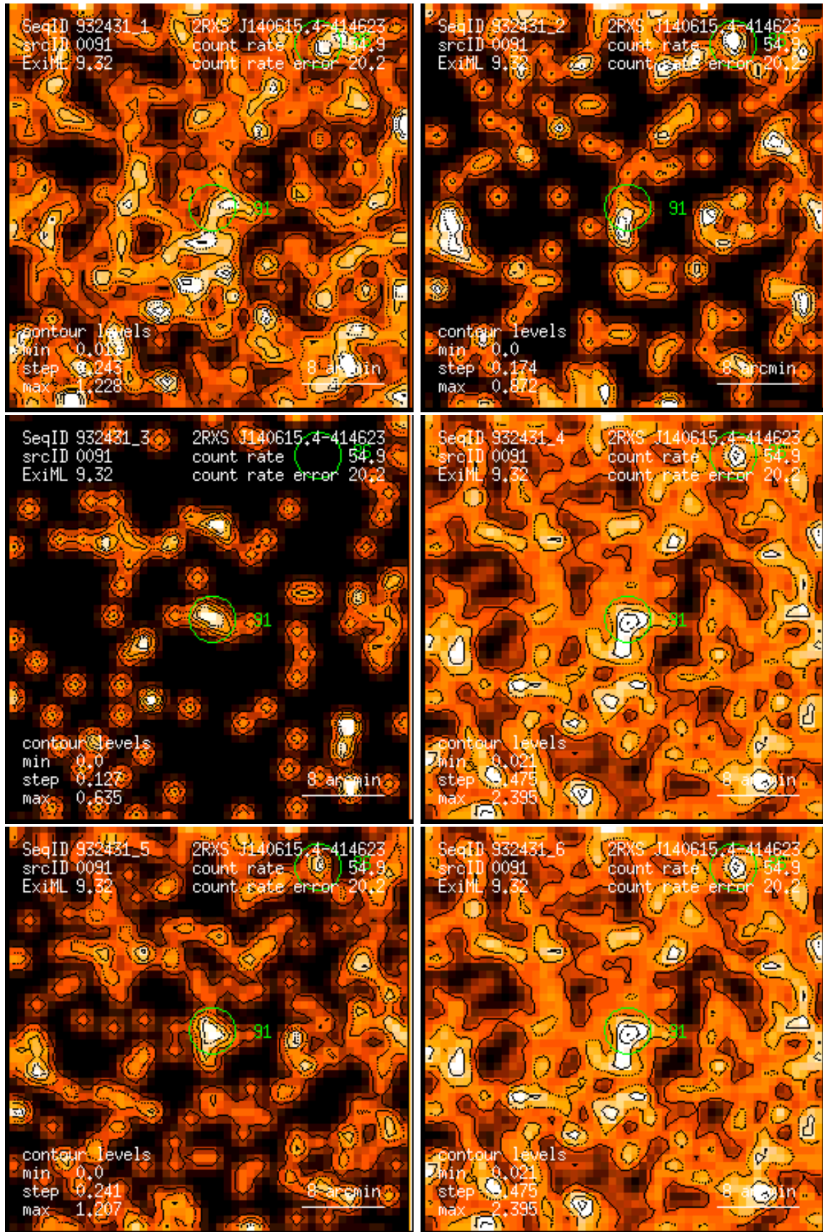
Figure 91: RASS 932431: detection 0091: band rate images, Gaussian filter: (1) PSPC channels 11 – 41, (2) 52 – 90, (3) 91 – 201, (4) 11 – 235, (5) 52 – 201, (6) 11 – 201. Broad band rates in counts/ks. Band rate contour levels in counts/ks/arcmin 2 .
