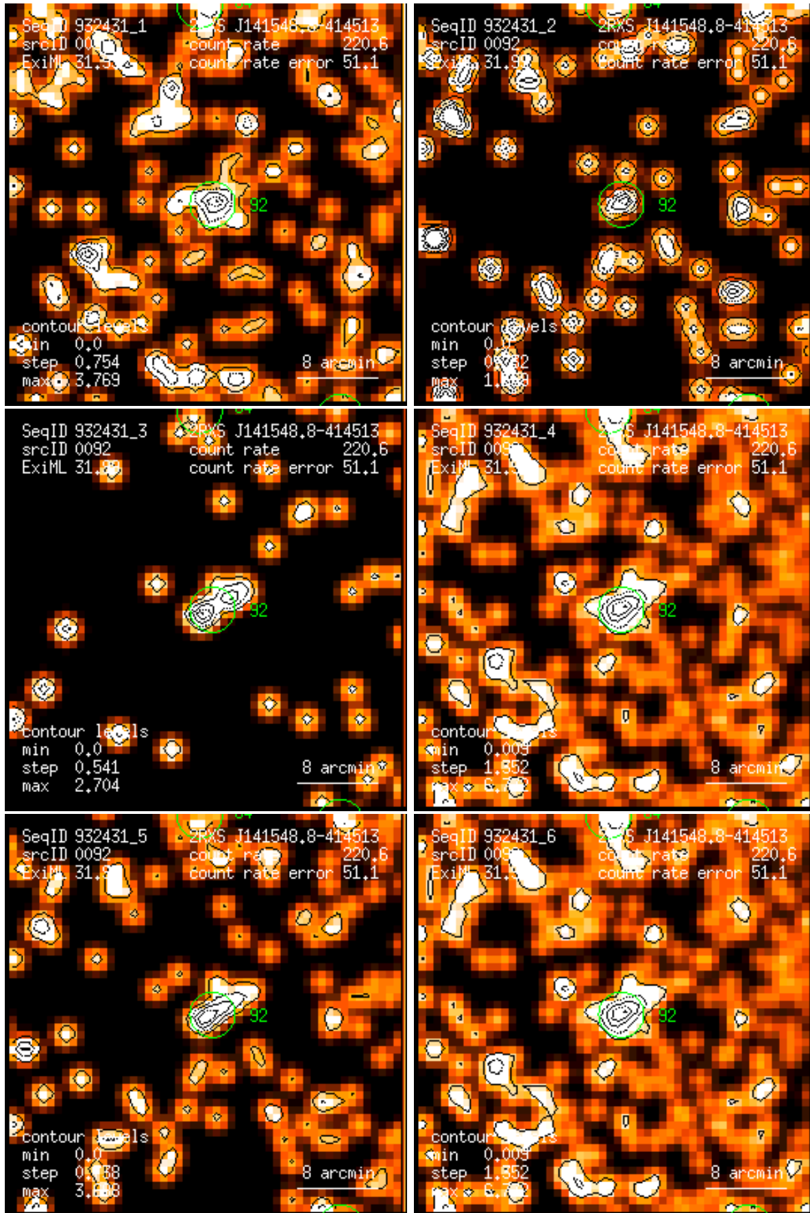
Figure 92: RASS 932431: detection 0092: band rate images, Gaussian filter: (1) PSPC channels 11 – 41, (2) 52 – 90, (3) 91 – 201, (4) 11 – 235, (5) 52 – 201, (6) 11 – 201. Broad band rates in counts/ks. Band rate contour levels in counts/ks/arcmin 2 .
