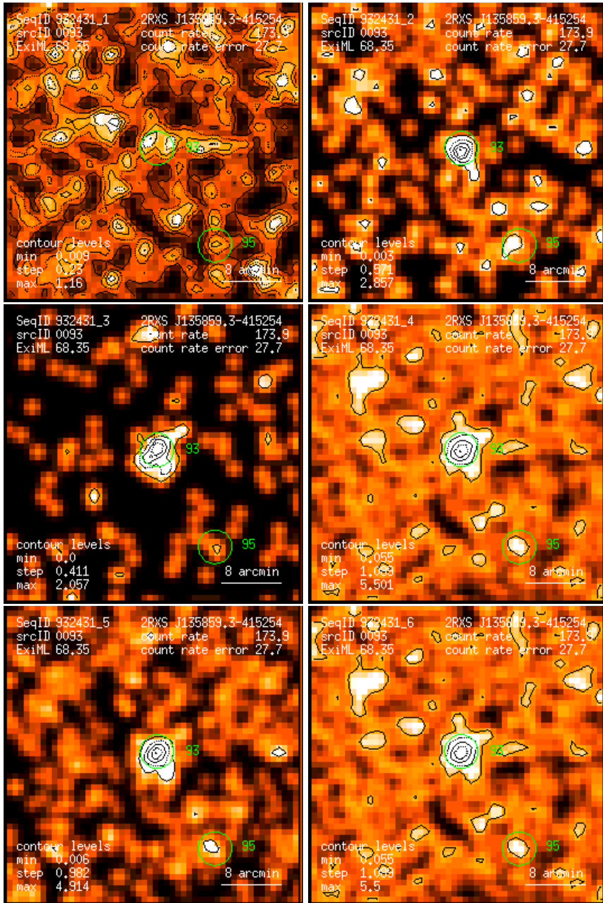
Figure 93: RASS 932431: detection 0093: band rate images, Gaussian filter: (1) PSPC channels 11 – 41, (2) 52 – 90, (3) 91 – 201, (4) 11 – 235, (5) 52 – 201, (6) 11 – 201. Broad band rates in counts/ks. Band rate contour levels in counts/ks/arcmin 2 .
