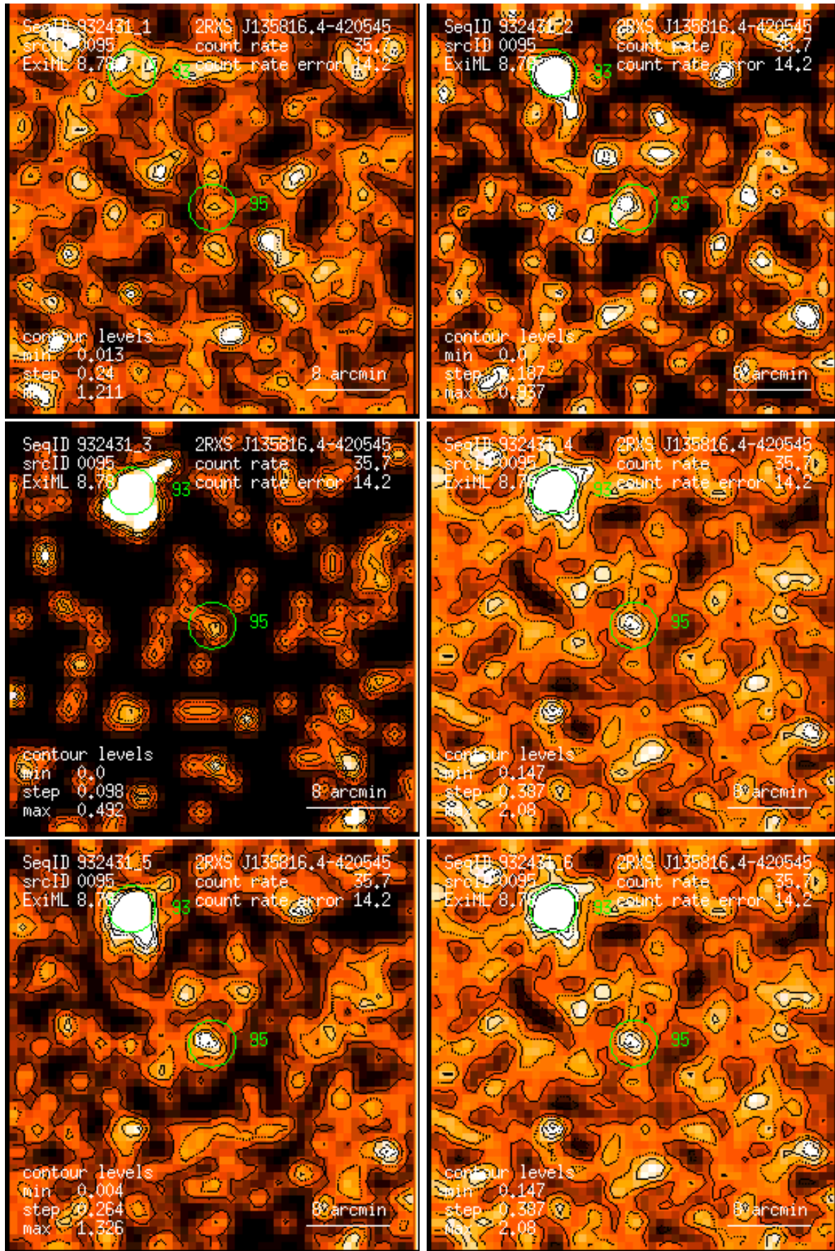
Figure 95: RASS 932431: detection 0095: band rate images, Gaussian filter: (1) PSPC channels 11 – 41, (2) 52 – 90, (3) 91 – 201, (4) 11 – 235, (5) 52 – 201, (6) 11 – 201. Broad band rates in counts/ks. Band rate contour levels in counts/ks/arcmin 2 .
