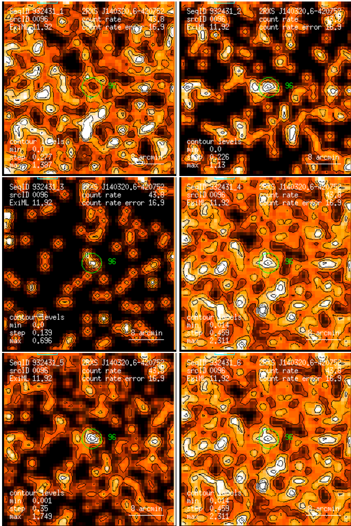
Figure 96: RASS 932431: detection 0096: band rate images, Gaussian filter: (1) PSPC channels 11 – 41, (2) 52 – 90, (3) 91 – 201, (4) 11 – 235, (5) 52 – 201, (6) 11 – 201. Broad band rates in counts/ks. Band rate contour levels in counts/ks/arcmin 2 .
