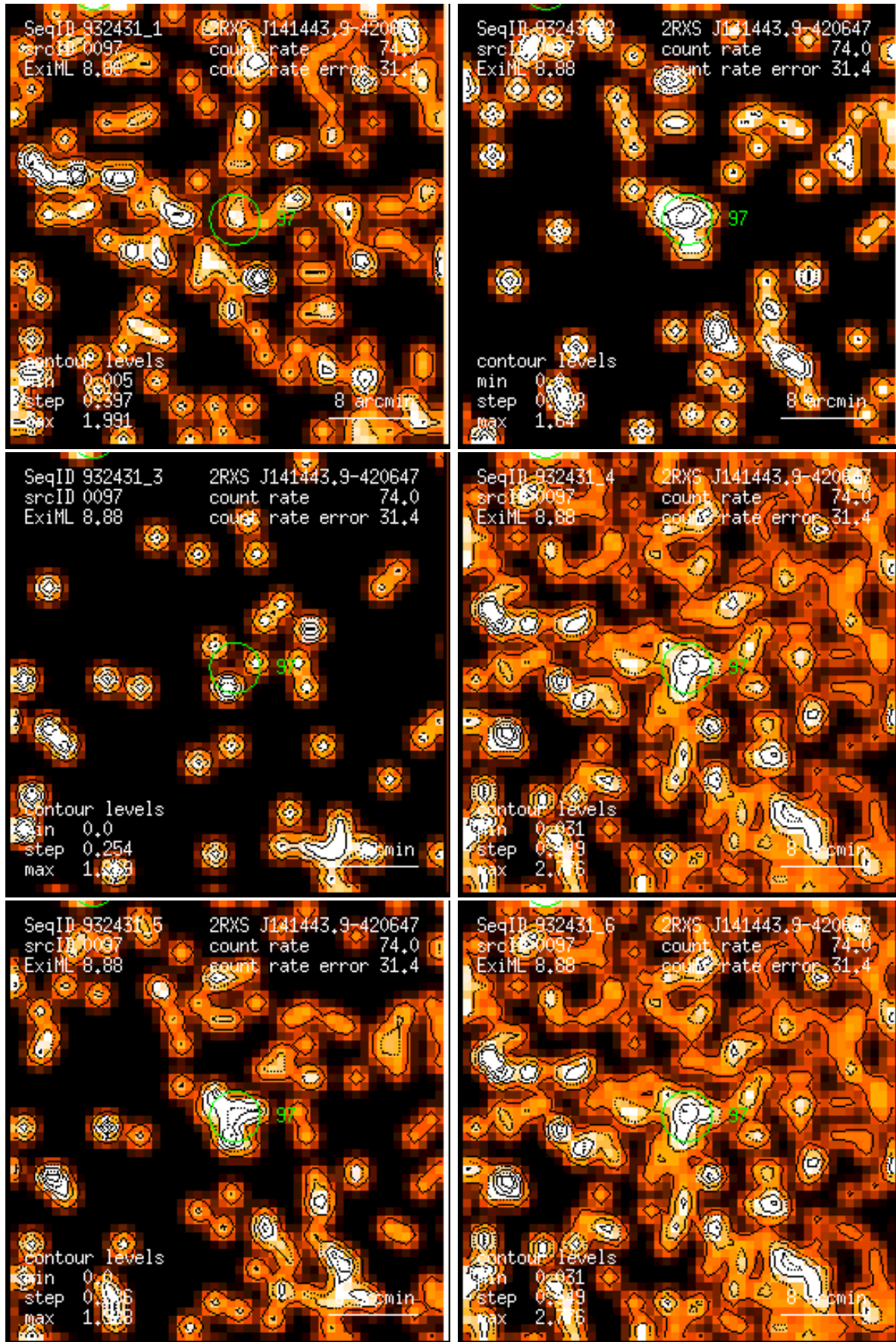
Figure 97: RASS 932431: detection 0097: band rate images, Gaussian filter: (1) PSPC channels 11 – 41, (2) 52 – 90, (3) 91 – 201, (4) 11 – 235, (5) 52 – 201, (6) 11 – 201. Broad band rates in counts/ks. Band rate contour levels in counts/ks/arcmin 2 .
