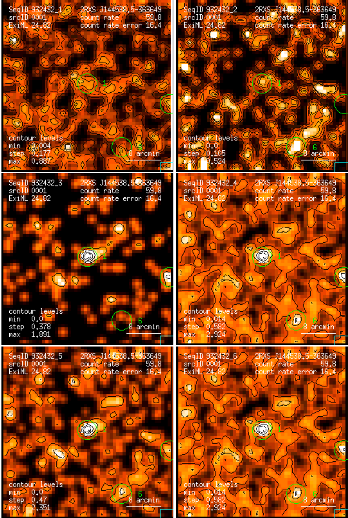
Figure 1: RASS 932432: detection 0001: band rate images, Gaussian filter: (1) PSPC channels 11 – 41, (2) 52 – 90, (3) 91 – 201, (4) 11 – 235, (5) 52 – 201, (6) 11 – 201. Broad band rates in counts/ks. Band rate contour levels in counts/ks/arcmin 2 .
