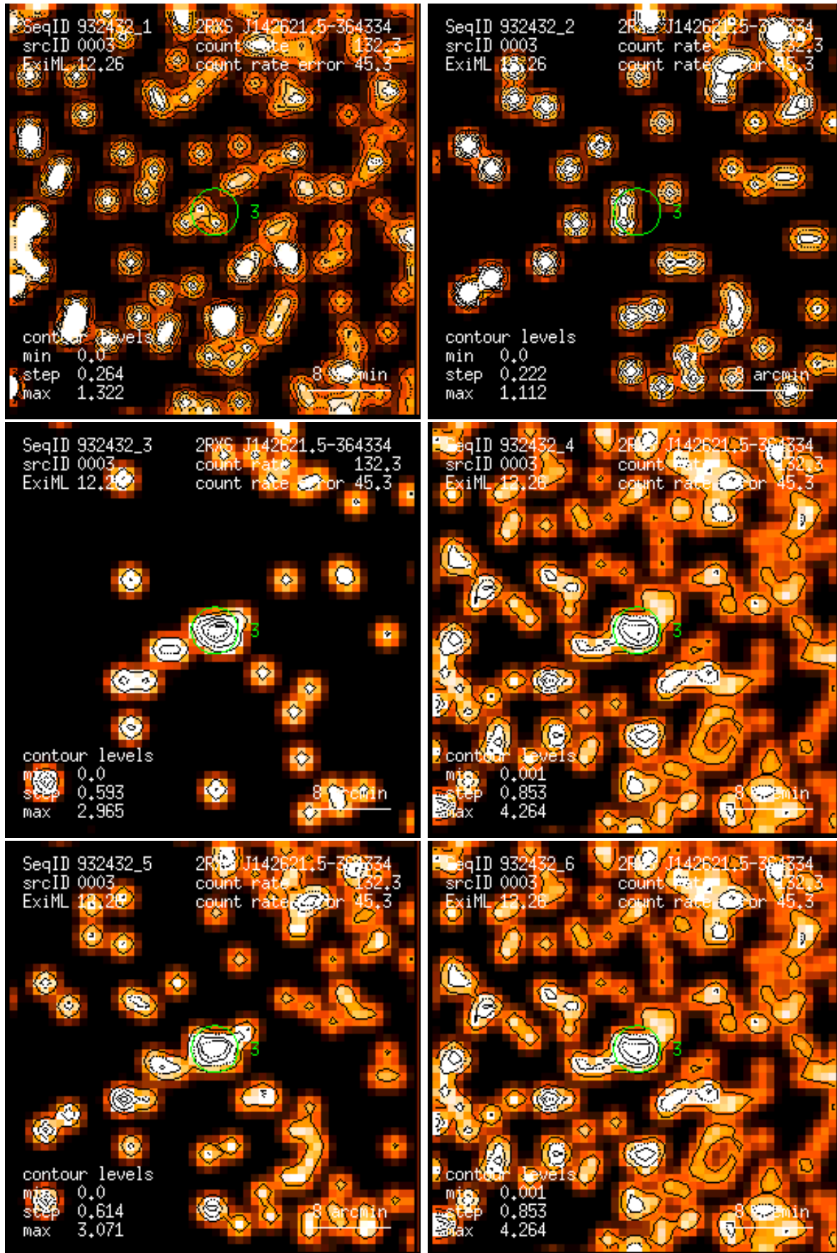
Figure 3: RASS 932432: detection 0003: band rate images, Gaussian filter: (1) PSPC channels 11 – 41, (2) 52 – 90, (3) 91 – 201, (4) 11 – 235, (5) 52 – 201, (6) 11 – 201. Broad band rates in counts/ks. Band rate contour levels in counts/ks/arcmin 2 .
