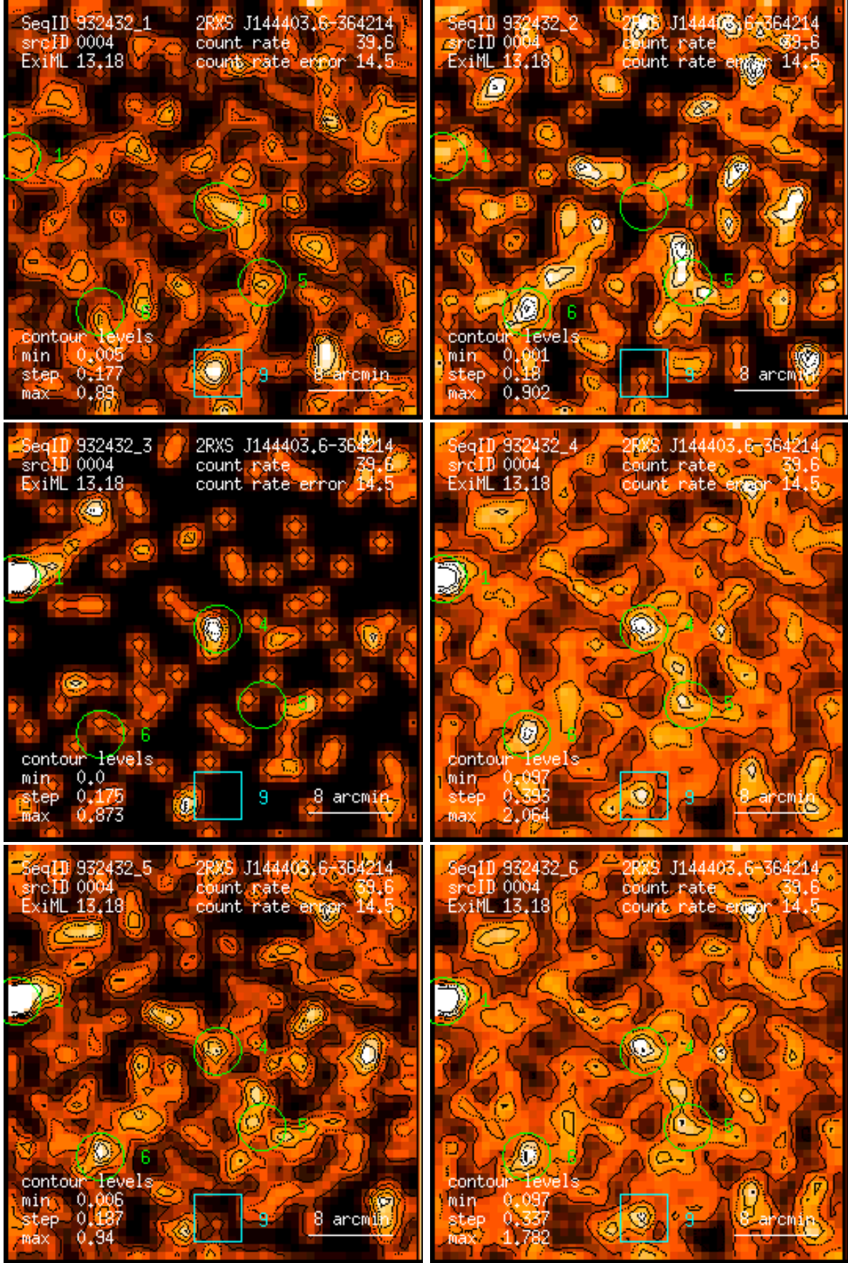
Figure 4: RASS 932432: detection 0004: band rate images, Gaussian filter: (1) PSPC channels 11 – 41, (2) 52 – 90, (3) 91 – 201, (4) 11 – 235, (5) 52 – 201, (6) 11 – 201. Broad band rates in counts/ks. Band rate contour levels in counts/ks/arcmin 2 .
