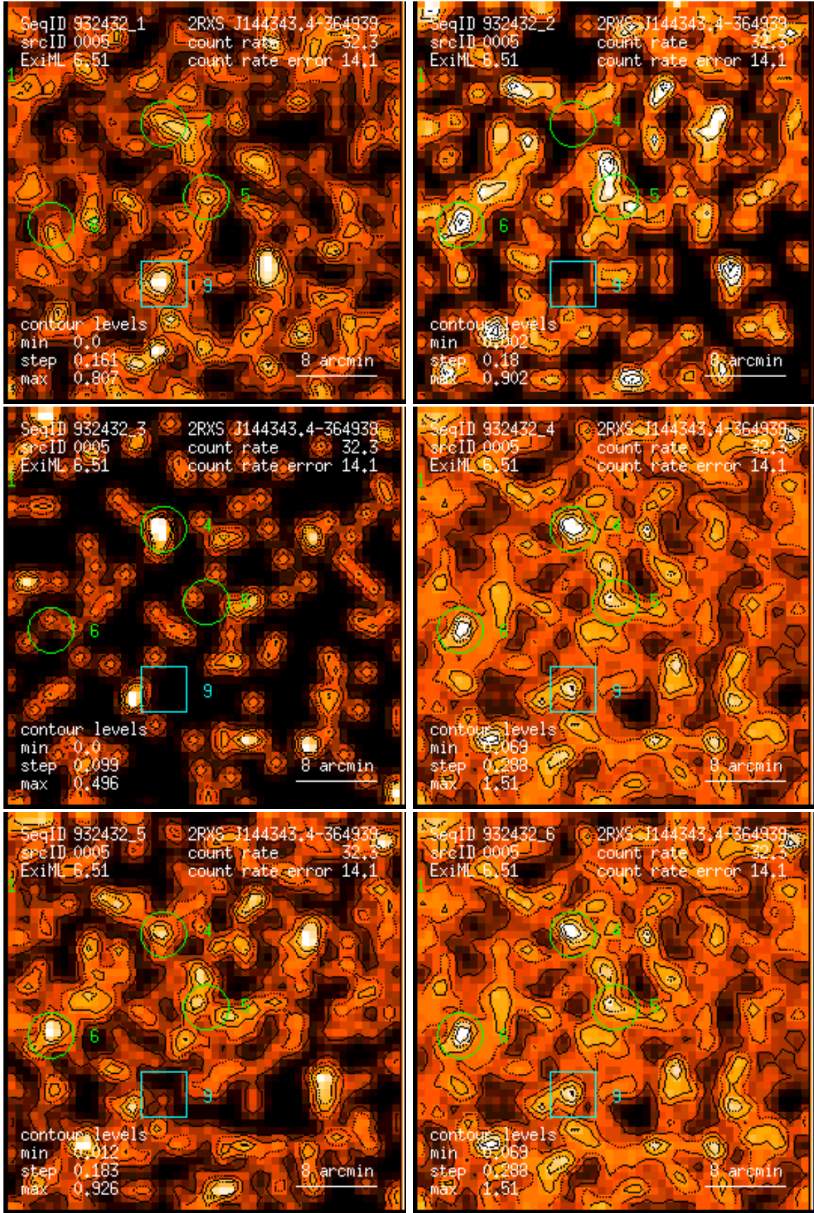
Figure 5: RASS 932432: detection 0005: band rate images, Gaussian filter: (1) PSPC channels 11 – 41, (2) 52 – 90, (3) 91 – 201, (4) 11 – 235, (5) 52 – 201, (6) 11 – 201. Broad band rates in counts/ks. Band rate contour levels in counts/ks/arcmin 2 .
