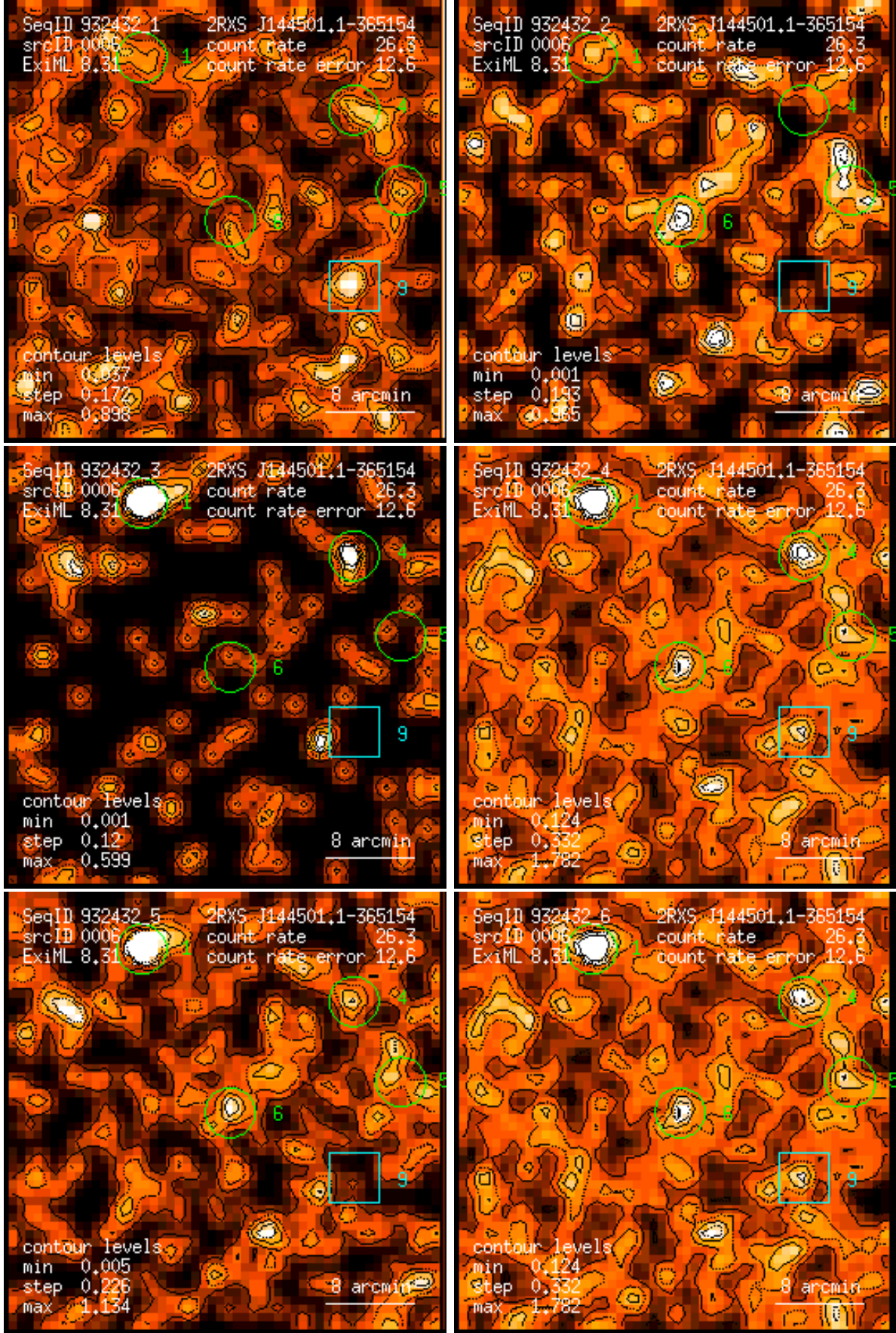
Figure 6: RASS 932432: detection 0006: band rate images, Gaussian filter: (1) PSPC channels 11 – 41, (2) 52 – 90, (3) 91 – 201, (4) 11 – 235, (5) 52 – 201, (6) 11 – 201. Broad band rates in counts/ks. Band rate contour levels in counts/ks/arcmin 2 .
