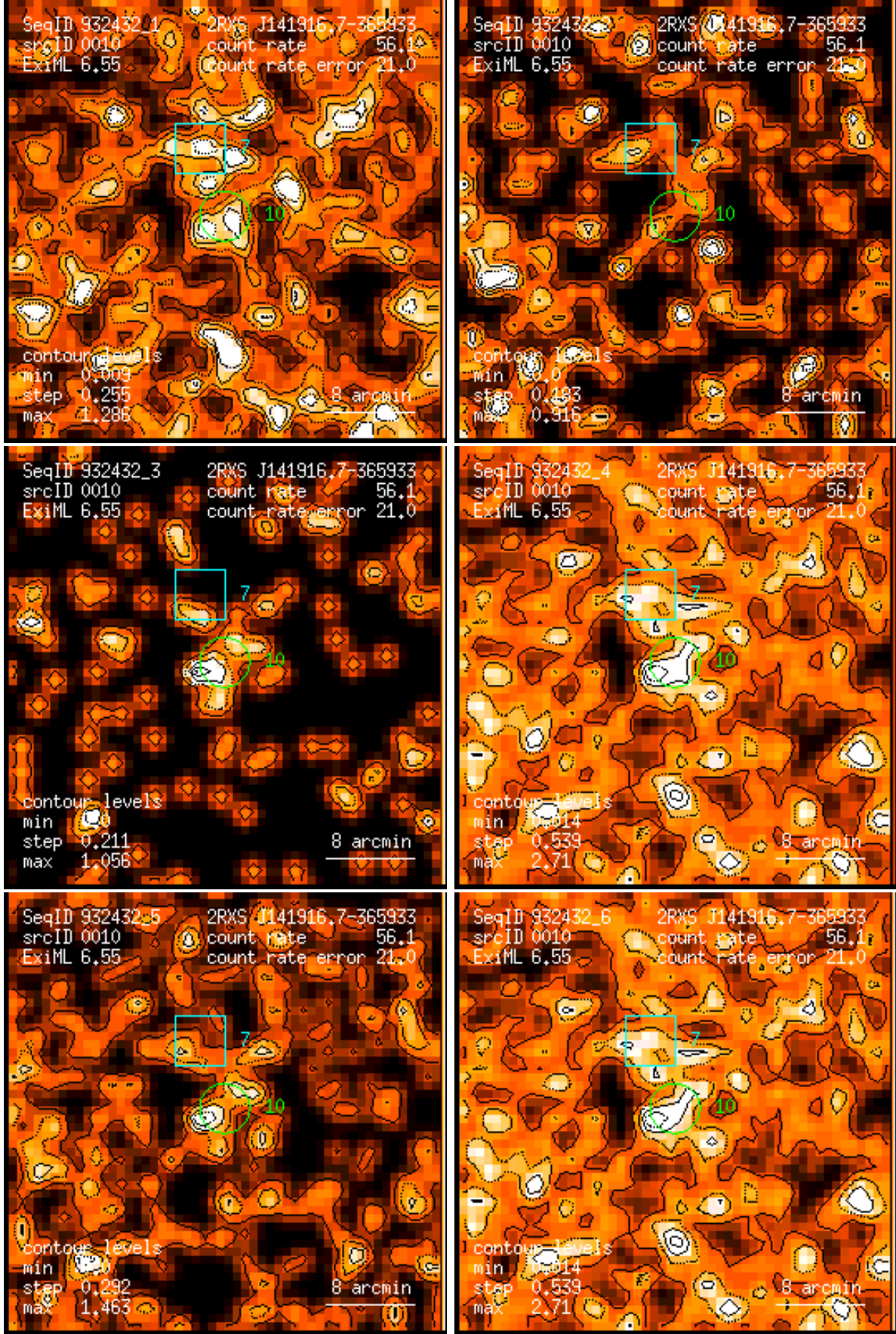
Figure 10: RASS 932432: detection 0010: band rate images, Gaussian filter: (1) PSPC channels 11 – 41, (2) 52 – 90, (3) 91 – 201, (4) 11 – 235, (5) 52 – 201, (6) 11 – 201. Broad band rates in counts/ks. Band rate contour levels in counts/ks/arcmin 2 .
