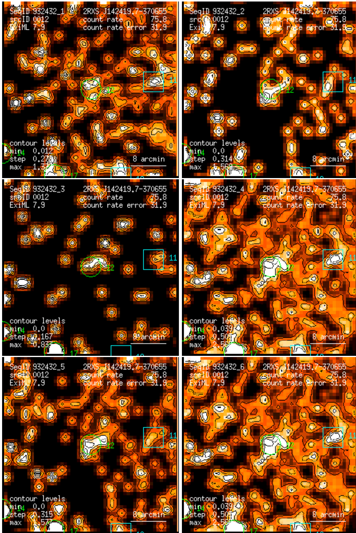
Figure 12: RASS 932432: detection 0012: band rate images, Gaussian filter: (1) PSPC channels 11 – 41, (2) 52 – 90, (3) 91 – 201, (4) 11 – 235, (5) 52 – 201, (6) 11 – 201. Broad band rates in counts/ks. Band rate contour levels in counts/ks/arcmin 2 .
