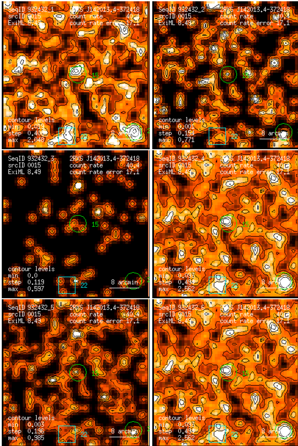
Figure 15: RASS 932432: detection 0015: band rate images, Gaussian filter: (1) PSPC channels 11 – 41, (2) 52 – 90, (3) 91 – 201, (4) 11 – 235, (5) 52 – 201, (6) 11 – 201. Broad band rates in counts/ks. Band rate contour levels in counts/ks/arcmin 2 .
