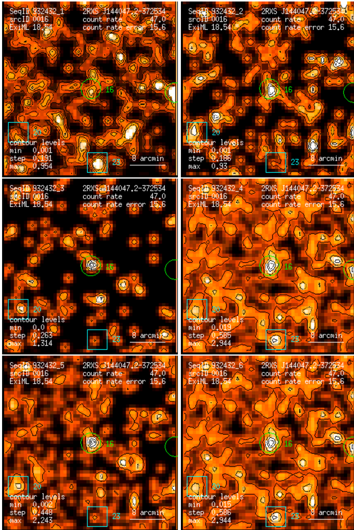
Figure 16: RASS 932432: detection 0016: band rate images, Gaussian filter: (1) PSPC channels 11 – 41, (2) 52 – 90, (3) 91 – 201, (4) 11 – 235, (5) 52 – 201, (6) 11 – 201. Broad band rates in counts/ks. Band rate contour levels in counts/ks/arcmin 2 .
