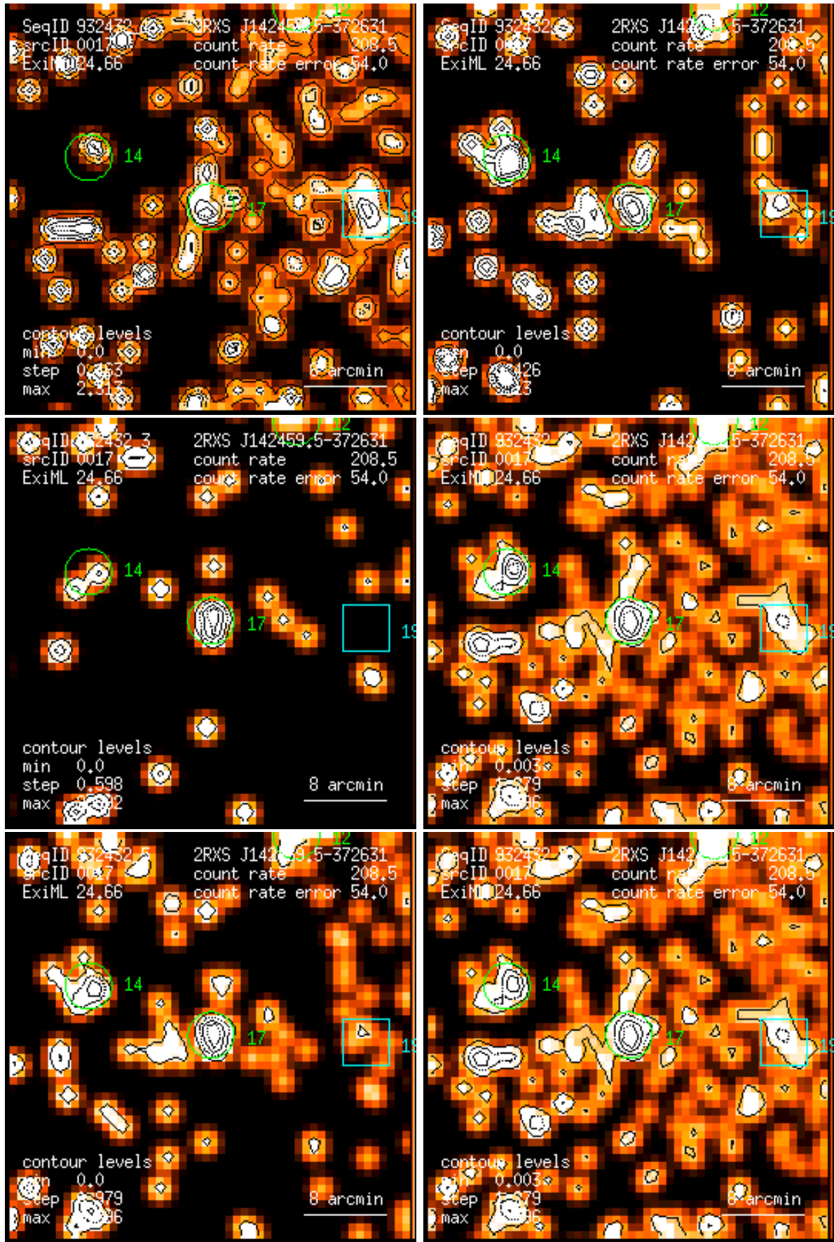
Figure 17: RASS 932432: detection 0017: band rate images, Gaussian filter: (1) PSPC channels 11 – 41, (2) 52 – 90, (3) 91 – 201, (4) 11 – 235, (5) 52 – 201, (6) 11 – 201. Broad band rates in counts/ks. Band rate contour levels in counts/ks/arcmin 2 .
