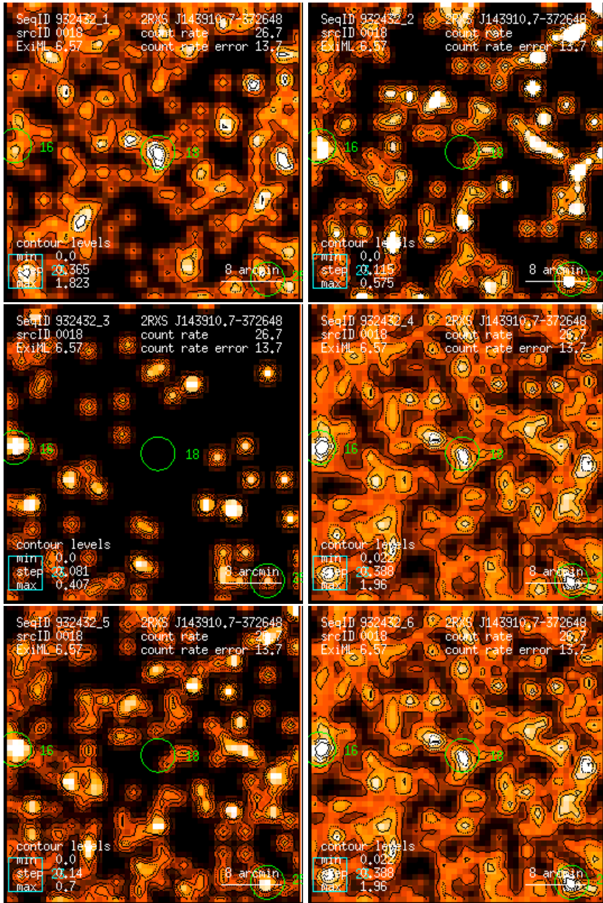
Figure 18: RASS 932432: detection 0018: band rate images, Gaussian filter: (1) PSPC channels 11 – 41, (2) 52 – 90, (3) 91 – 201, (4) 11 – 235, (5) 52 – 201, (6) 11 – 201. Broad band rates in counts/ks. Band rate contour levels in counts/ks/arcmin 2 .
