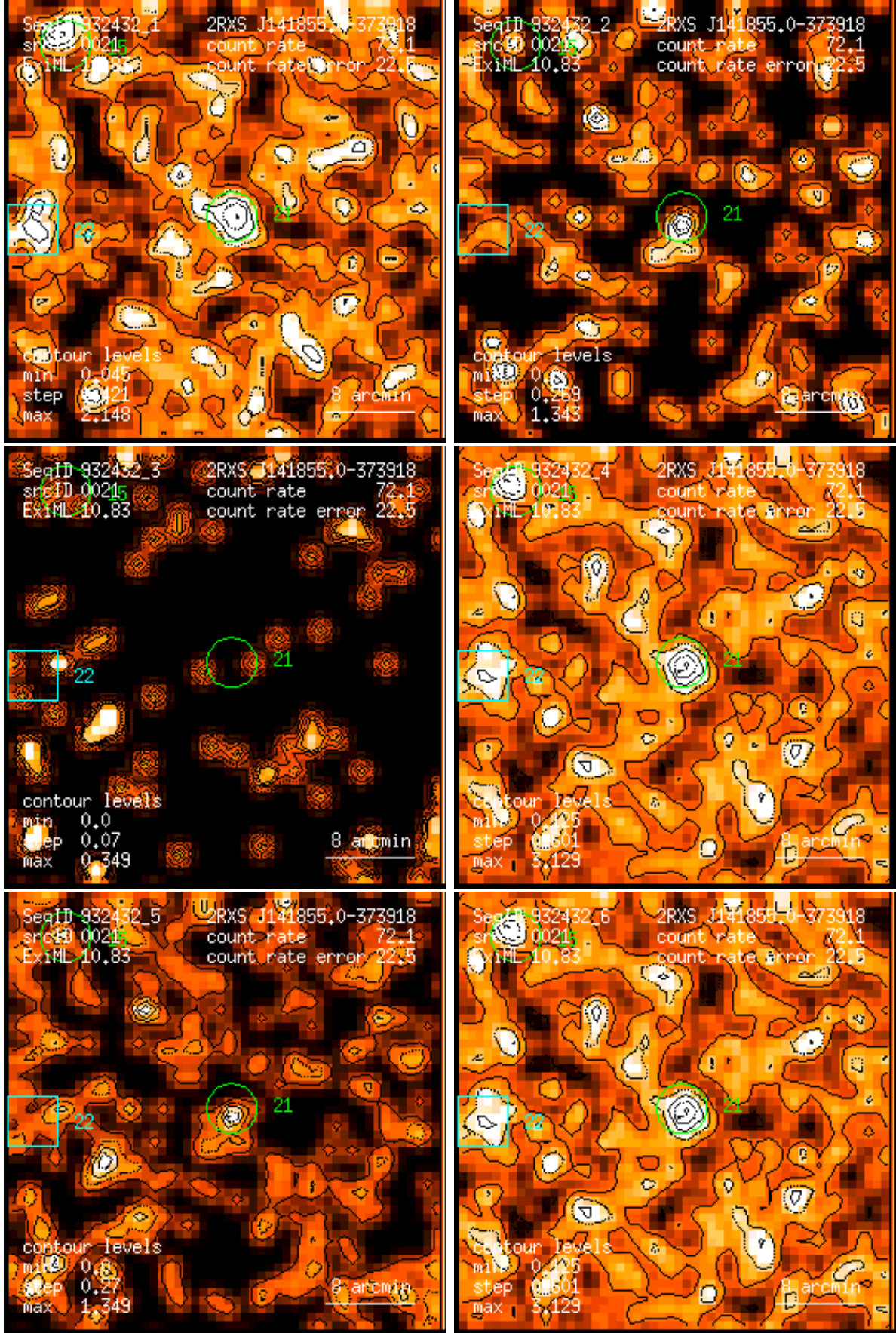
Figure 21: RASS 932432: detection 0021: band rate images, Gaussian filter: (1) PSPC channels 11 – 41, (2) 52 – 90, (3) 91 – 201, (4) 11 – 235, (5) 52 – 201, (6) 11 – 201. Broad band rates in counts/ks. Band rate contour levels in counts/ks/arcmin 2 .
