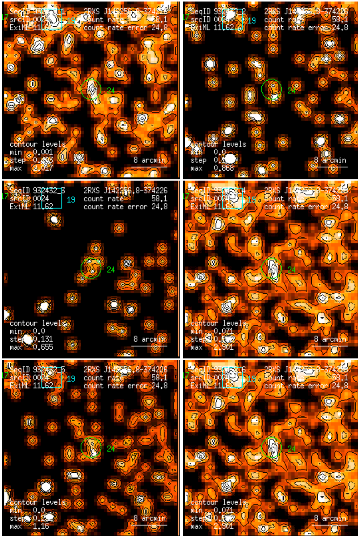
Figure 24: RASS 932432: detection 0024: band rate images, Gaussian filter: (1) PSPC channels 11 – 41, (2) 52 – 90, (3) 91 – 201, (4) 11 – 235, (5) 52 – 201, (6) 11 – 201. Broad band rates in counts/ks. Band rate contour levels in counts/ks/arcmin 2 .
