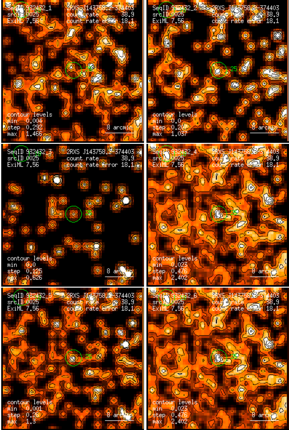
Figure 25: RASS 932432: detection 0025: band rate images, Gaussian filter: (1) PSPC channels 11 – 41, (2) 52 – 90, (3) 91 – 201, (4) 11 – 235, (5) 52 – 201, (6) 11 – 201. Broad band rates in counts/ks. Band rate contour levels in counts/ks/arcmin 2 .
