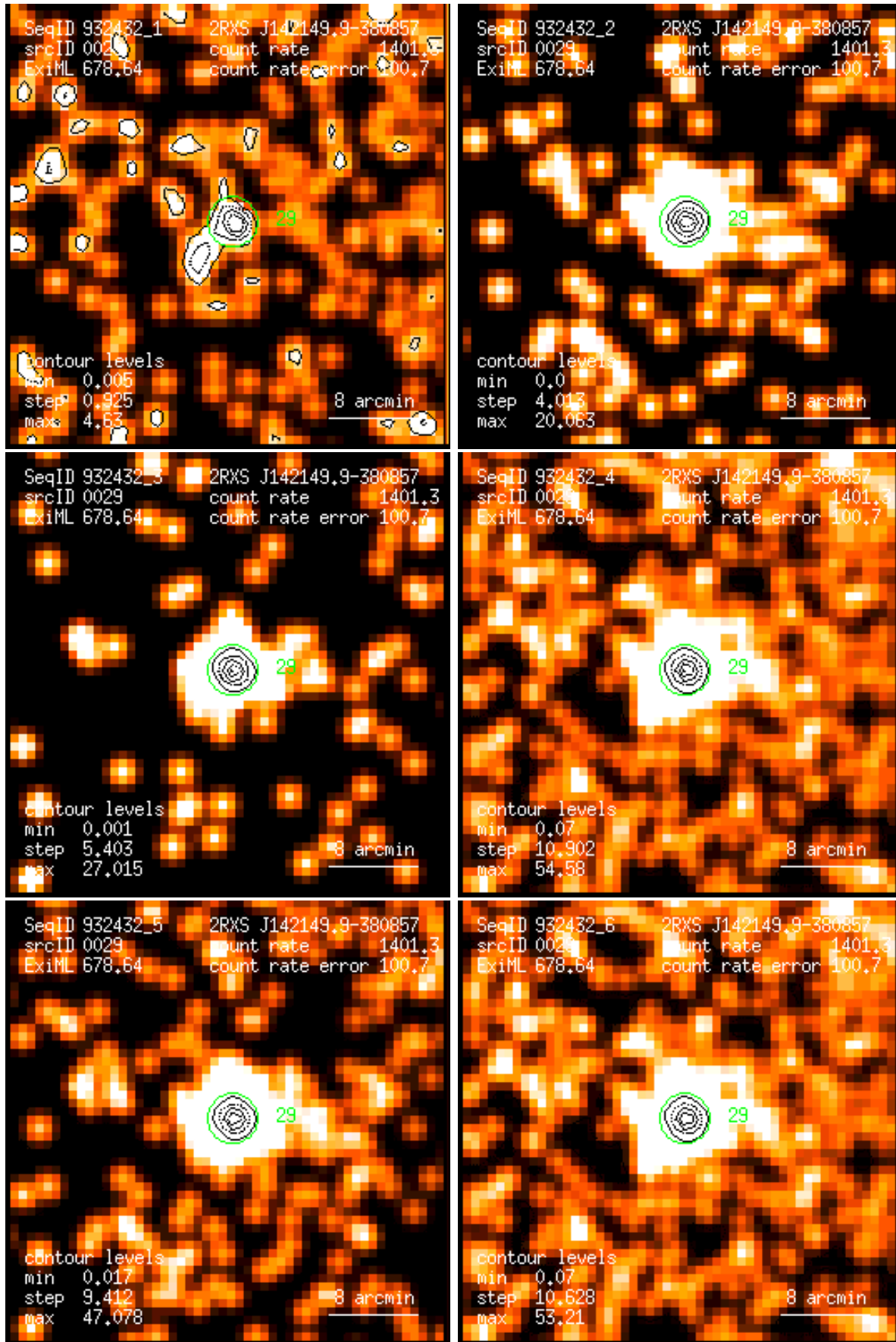
Figure 29: RASS 932432: detection 0029: band rate images, Gaussian filter: (1) PSPC channels 11 – 41, (2) 52 – 90, (3) 91 – 201, (4) 11 – 235, (5) 52 – 201, (6) 11 – 201. Broad band rates in counts/ks. Band rate contour levels in counts/ks/arcmin 2 .
