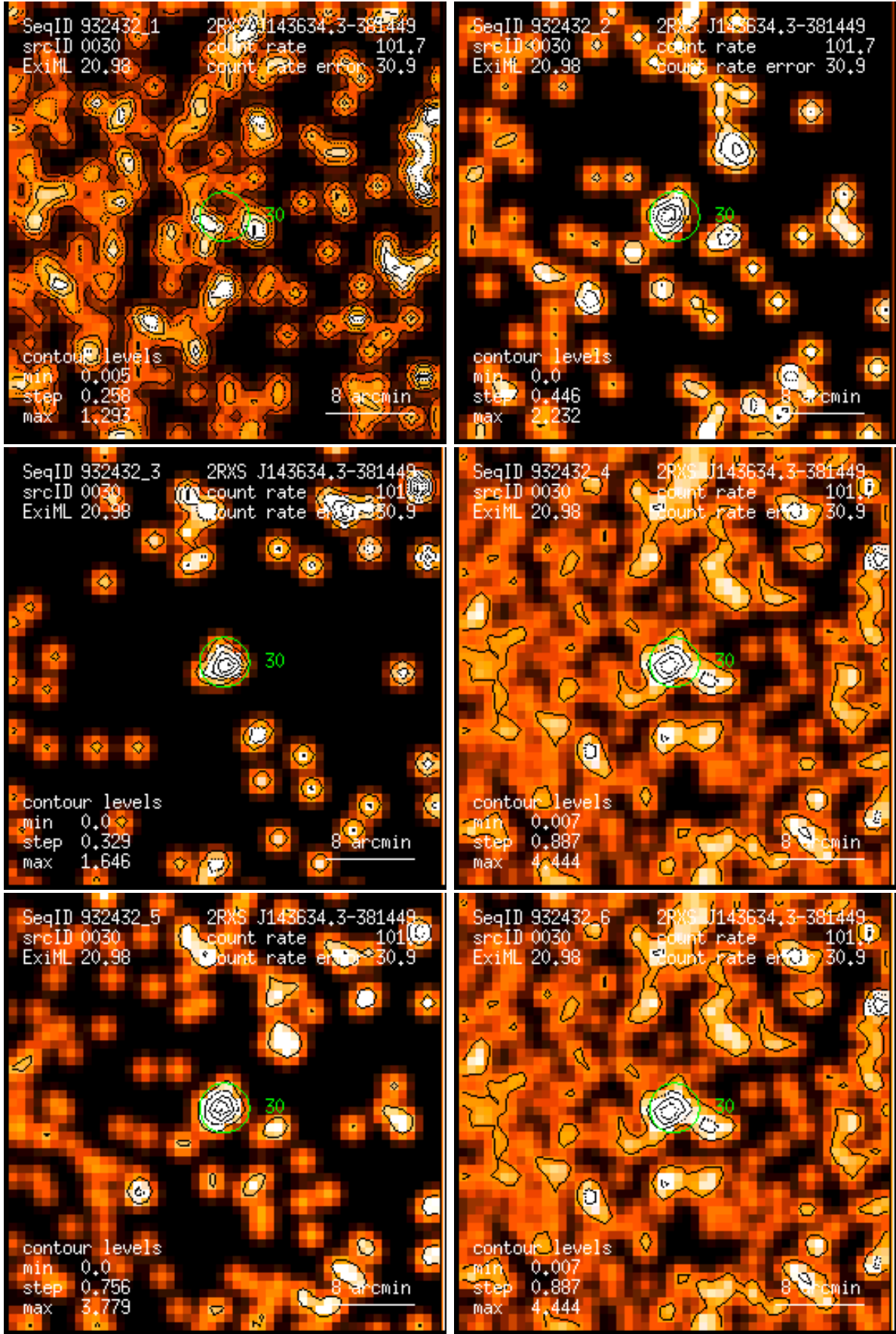
Figure 30: RASS 932432: detection 0030: band rate images, Gaussian filter: (1) PSPC channels 11 – 41, (2) 52 – 90, (3) 91 – 201, (4) 11 – 235, (5) 52 – 201, (6) 11 – 201. Broad band rates in counts/ks. Band rate contour levels in counts/ks/arcmin 2 .
