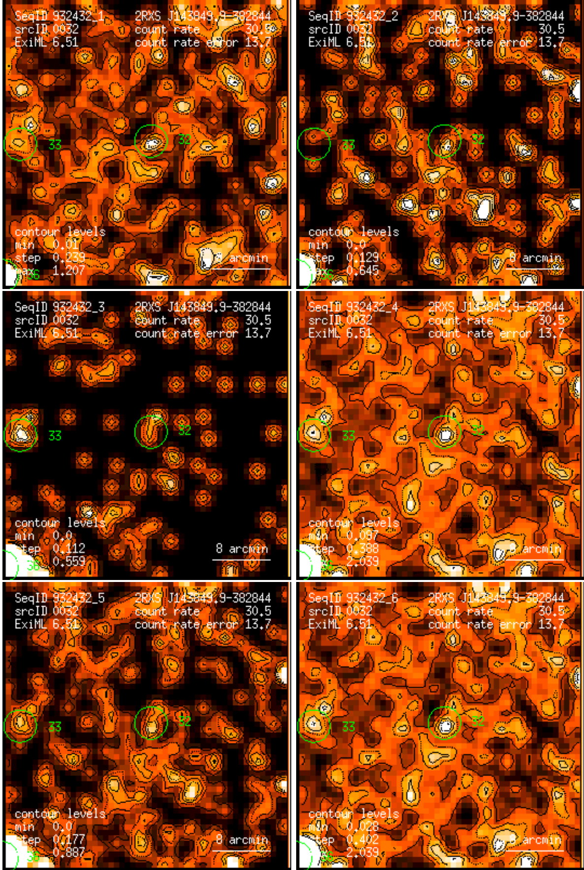
Figure 32: RASS 932432: detection 0032: band rate images, Gaussian filter: (1) PSPC channels 11 – 41, (2) 52 – 90, (3) 91 – 201, (4) 11 – 235, (5) 52 – 201, (6) 11 – 201. Broad band rates in counts/ks. Band rate contour levels in counts/ks/arcmin 2 .
