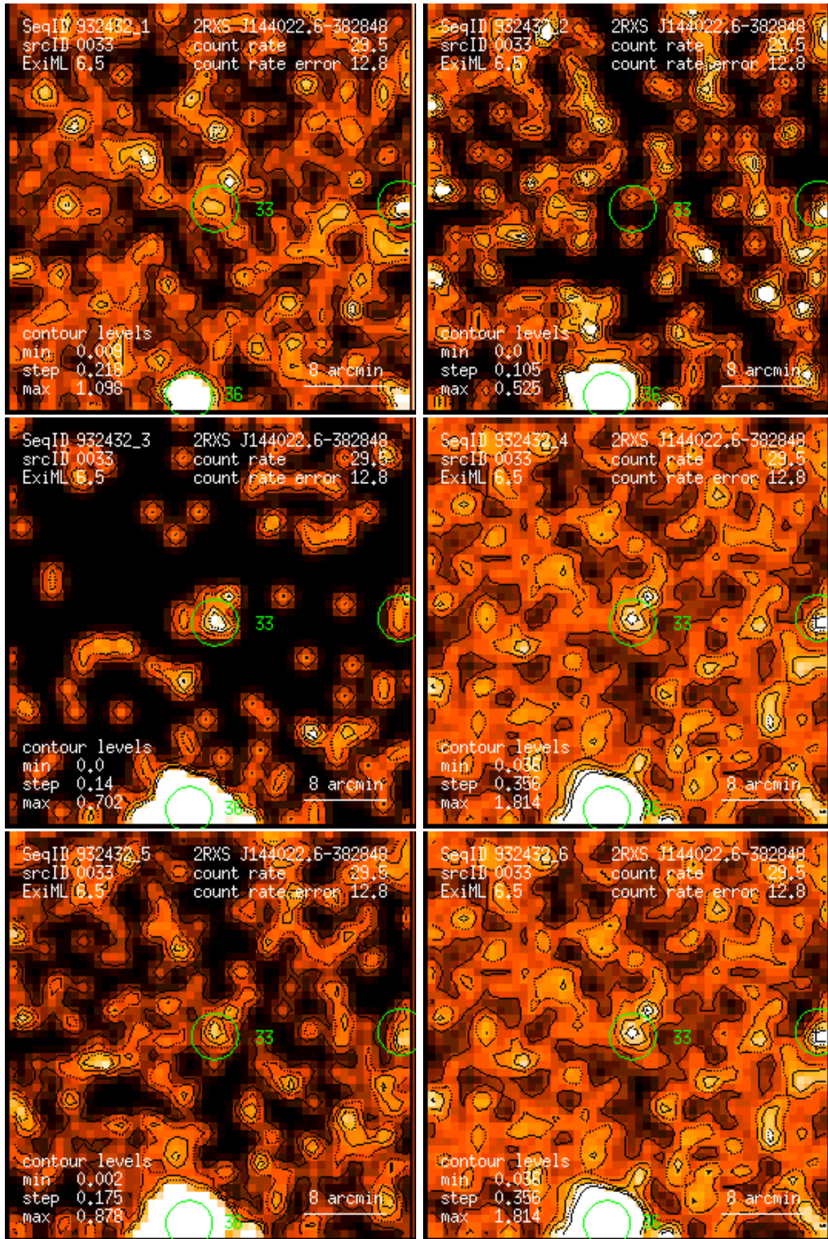
Figure 33: RASS 932432: detection 0033: band rate images, Gaussian filter: (1) PSPC channels 11 – 41, (2) 52 – 90, (3) 91 – 201, (4) 11 – 235, (5) 52 – 201, (6) 11 – 201. Broad band rates in counts/ks. Band rate contour levels in counts/ks/arcmin 2 .
