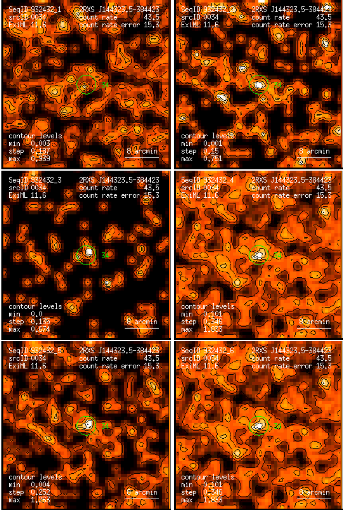
Figure 34: RASS 932432: detection 0034: band rate images, Gaussian filter: (1) PSPC channels 11 – 41, (2) 52 – 90, (3) 91 – 201, (4) 11 – 235, (5) 52 – 201, (6) 11 – 201. Broad band rates in counts/ks. Band rate contour levels in counts/ks/arcmin 2 .
