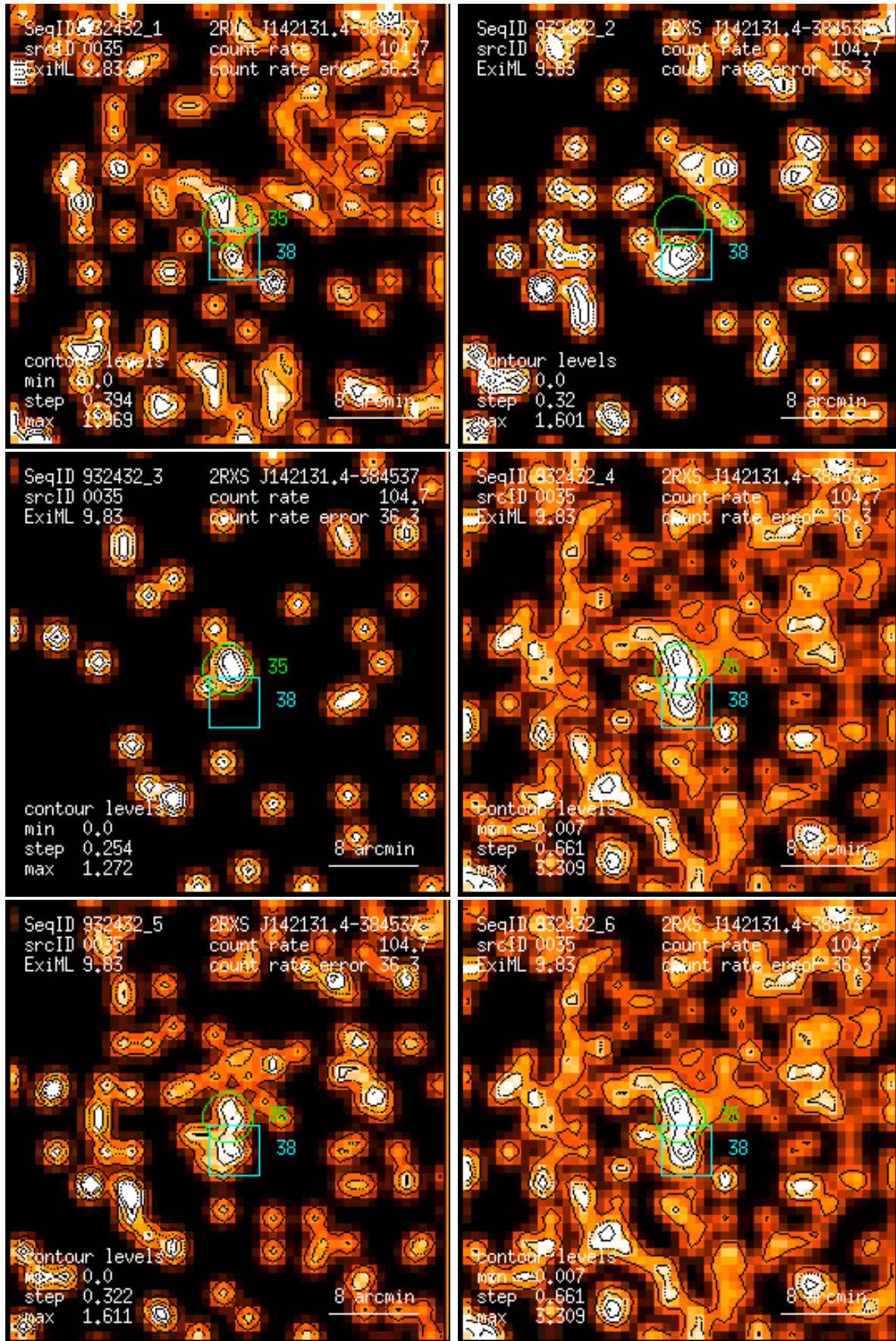
Figure 35: RASS 932432: detection 0035: band rate images, Gaussian filter: (1) PSPC channels 11 – 41, (2) 52 – 90, (3) 91 – 201, (4) 11 – 235, (5) 52 – 201, (6) 11 – 201. Broad band rates in counts/ks. Band rate contour levels in counts/ks/arcmin 2 .
