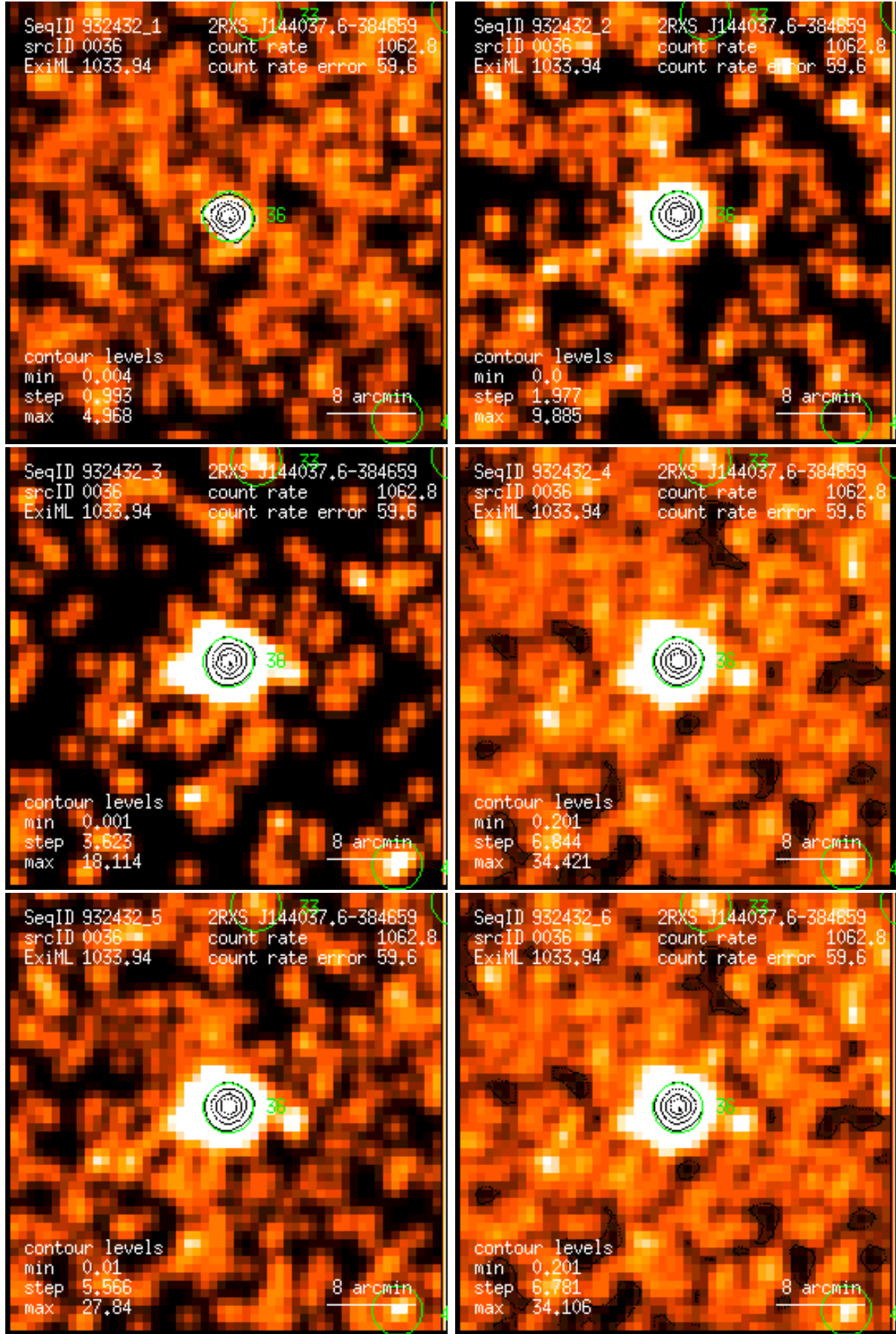
Figure 36: RASS 932432: detection 0036: band rate images, Gaussian filter: (1) PSPC channels 11 – 41, (2) 52 – 90, (3) 91 – 201, (4) 11 – 235, (5) 52 – 201, (6) 11 – 201. Broad band rates in counts/ks. Band rate contour levels in counts/ks/arcmin 2 .
