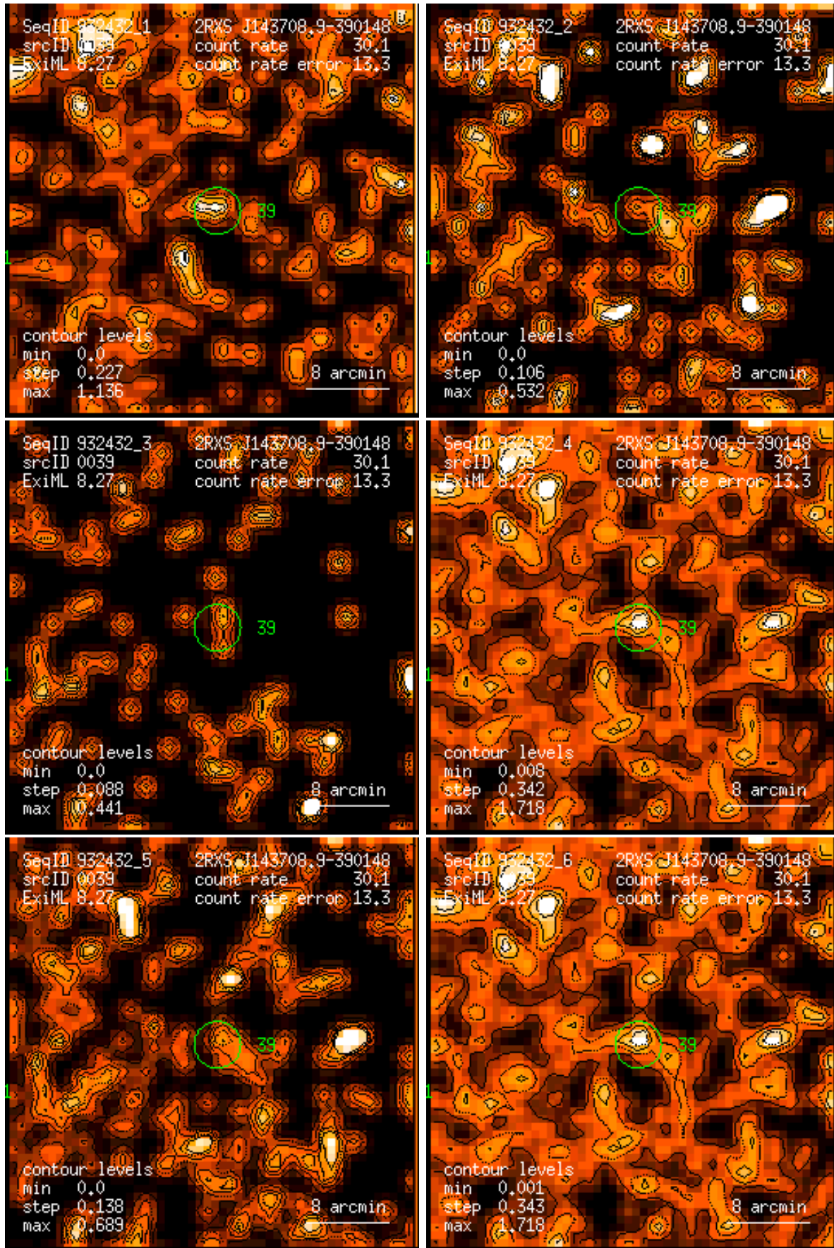
Figure 39: RASS 932432: detection 0039: band rate images, Gaussian filter: (1) PSPC channels 11 – 41, (2) 52 – 90, (3) 91 – 201, (4) 11 – 235, (5) 52 – 201, (6) 11 – 201. Broad band rates in counts/ks. Band rate contour levels in counts/ks/arcmin 2 .
