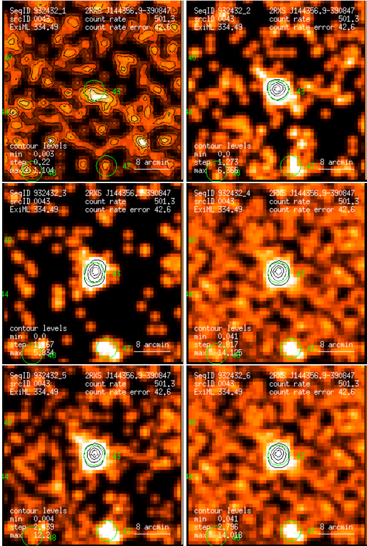
Figure 43: RASS 932432: detection 0043: band rate images, Gaussian filter: (1) PSPC channels 11 – 41, (2) 52 – 90, (3) 91 – 201, (4) 11 – 235, (5) 52 – 201, (6) 11 – 201. Broad band rates in counts/ks. Band rate contour levels in counts/ks/arcmin 2 .
