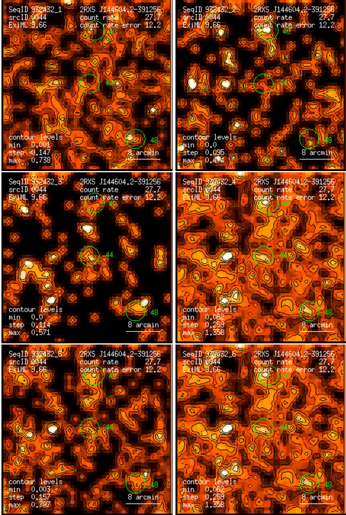
Figure 44: RASS 932432: detection 0044: band rate images, Gaussian filter: (1) PSPC channels 11 – 41, (2) 52 – 90, (3) 91 – 201, (4) 11 – 235, (5) 52 – 201, (6) 11 – 201. Broad band rates in counts/ks. Band rate contour levels in counts/ks/arcmin 2 .
