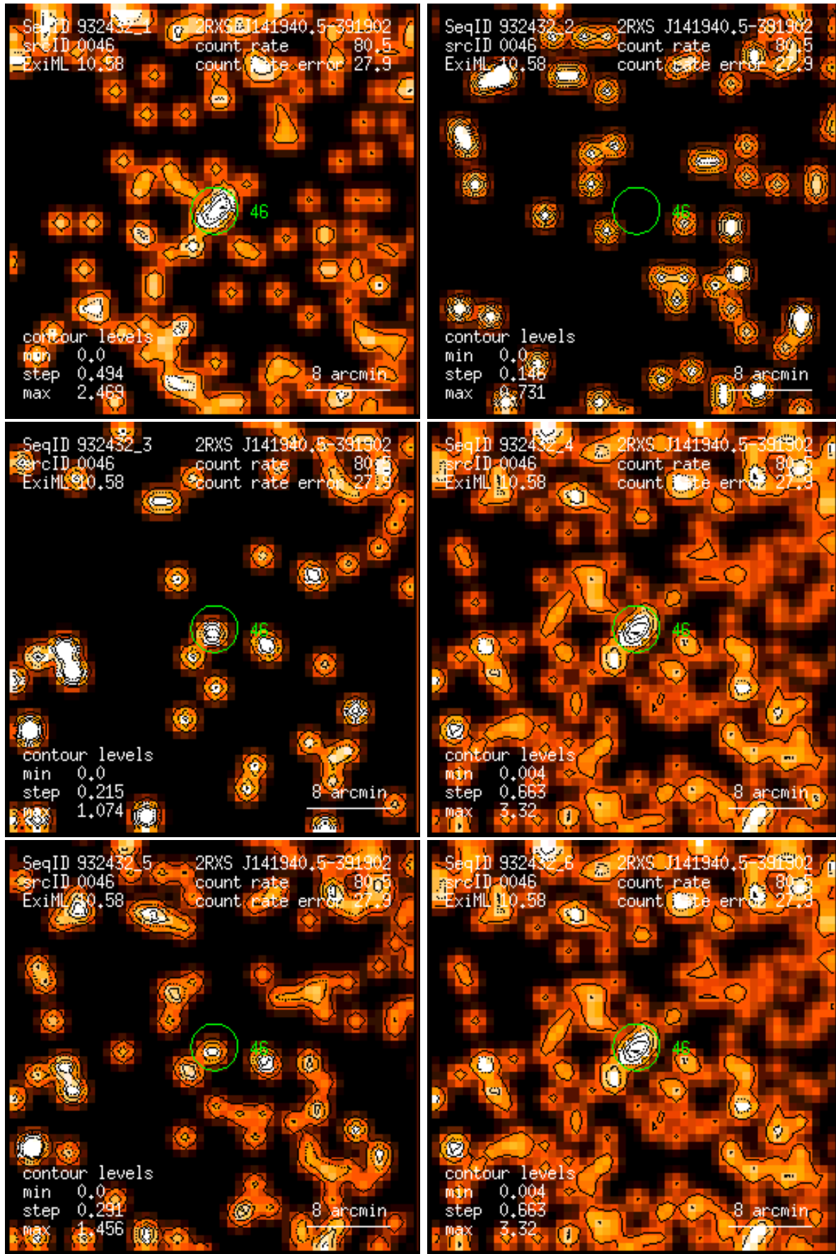
Figure 46: RASS 932432: detection 0046: band rate images, Gaussian filter: (1) PSPC channels 11 – 41, (2) 52 – 90, (3) 91 – 201, (4) 11 – 235, (5) 52 – 201, (6) 11 – 201. Broad band rates in counts/ks. Band rate contour levels in counts/ks/arcmin 2 .
