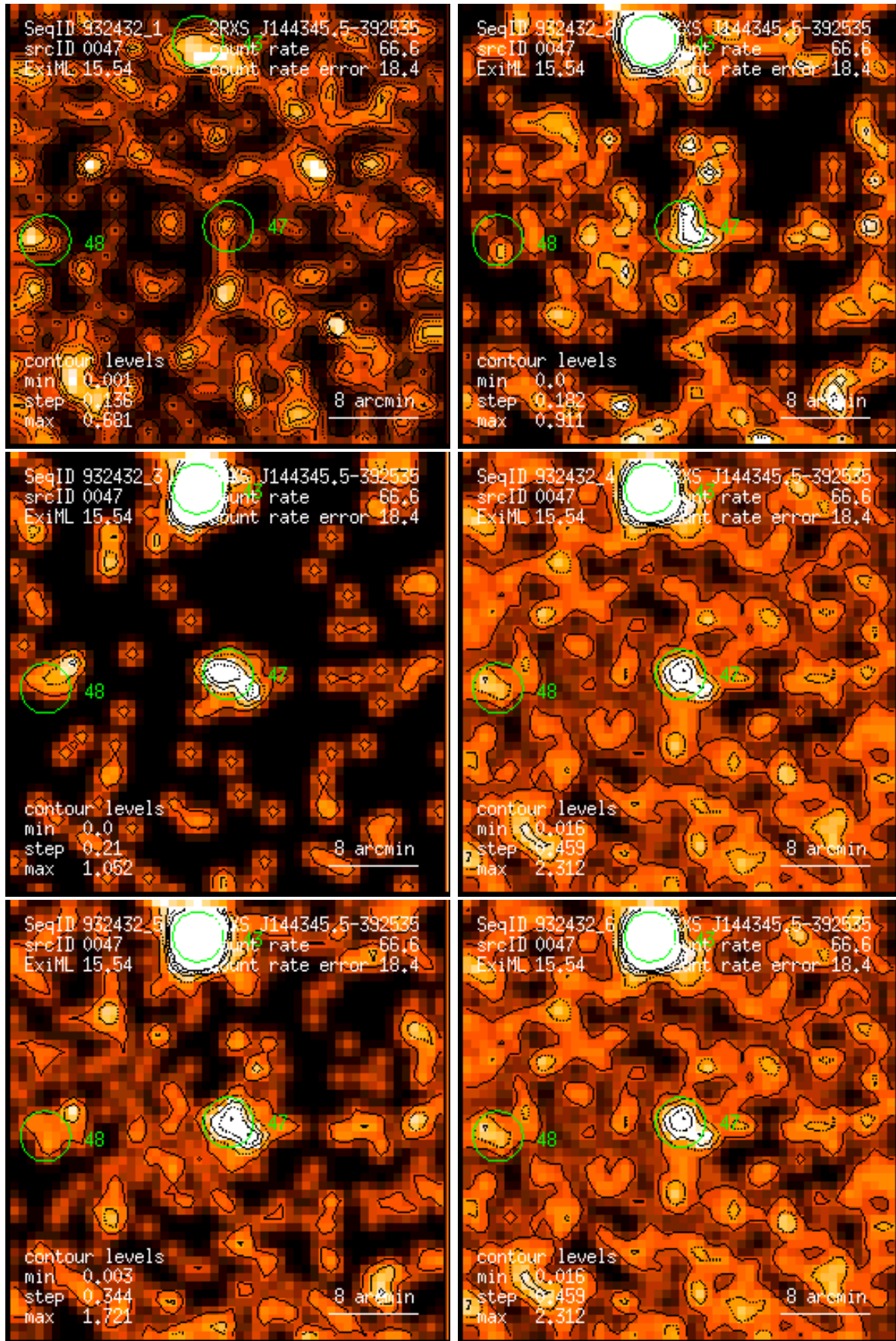
Figure 47: RASS 932432: detection 0047: band rate images, Gaussian filter: (1) PSPC channels 11 – 41, (2) 52 – 90, (3) 91 – 201, (4) 11 – 235, (5) 52 – 201, (6) 11 – 201. Broad band rates in counts/ks. Band rate contour levels in counts/ks/arcmin 2 .
