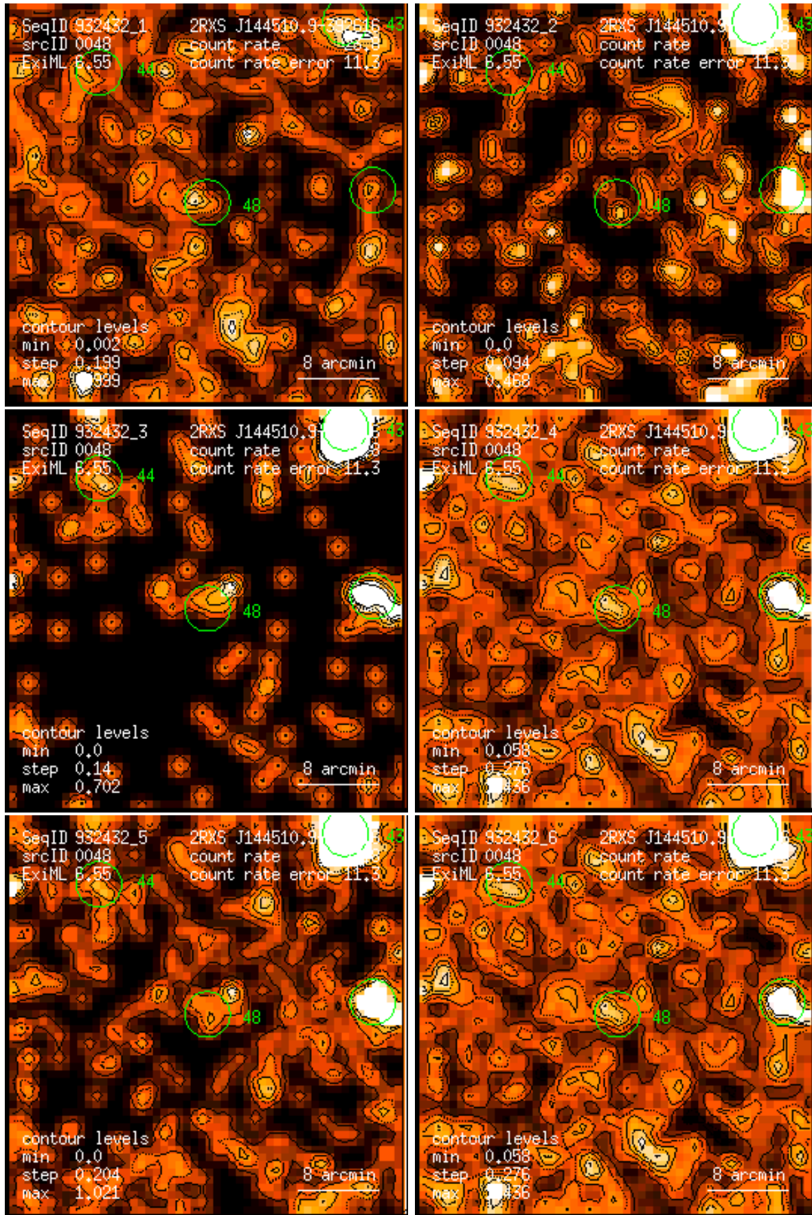
Figure 48: RASS 932432: detection 0048: band rate images, Gaussian filter: (1) PSPC channels 11 – 41, (2) 52 – 90, (3) 91 – 201, (4) 11 – 235, (5) 52 – 201, (6) 11 – 201. Broad band rates in counts/ks. Band rate contour levels in counts/ks/arcmin 2 .
