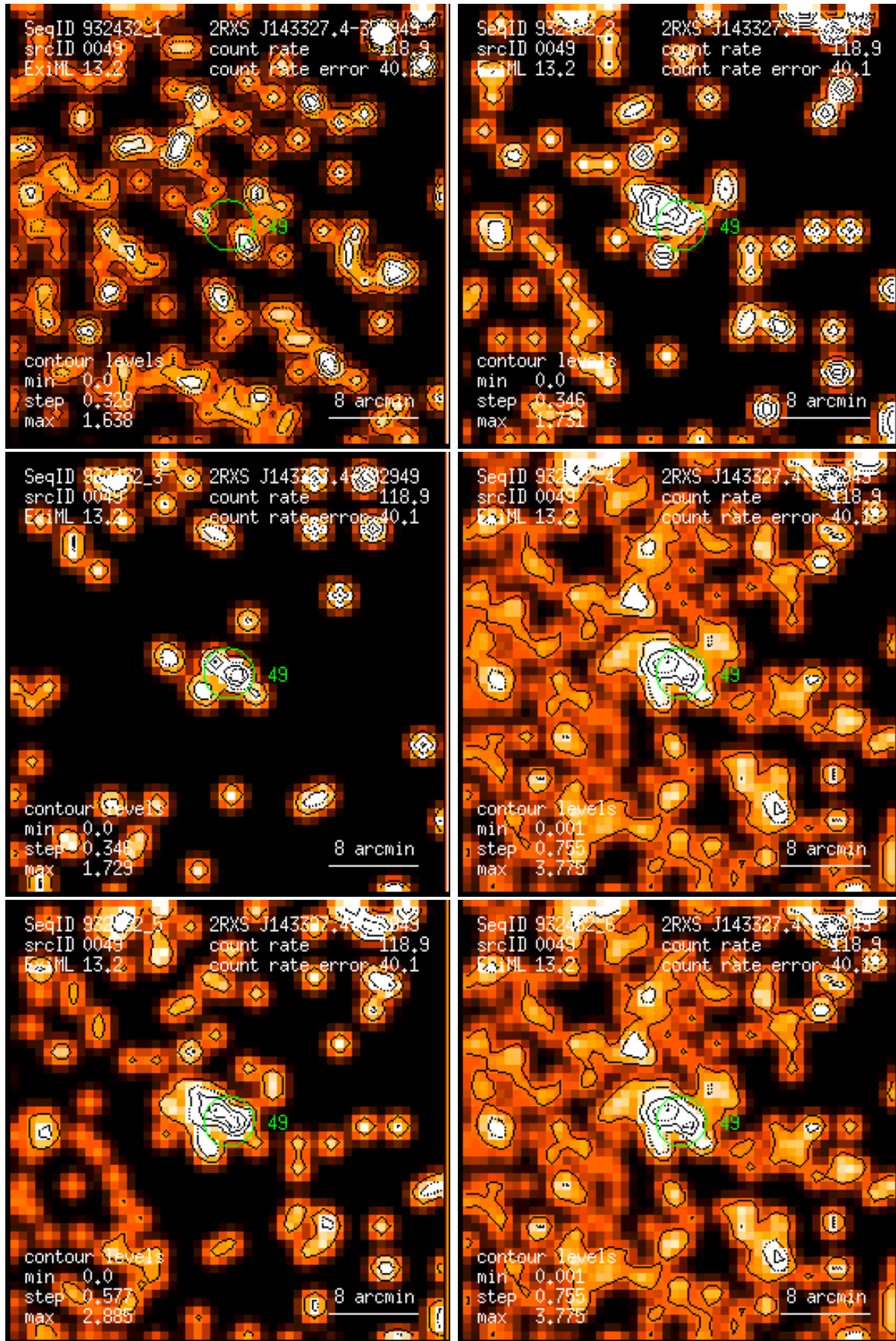
Figure 49: RASS 932432: detection 0049: band rate images, Gaussian filter: (1) PSPC channels 11 – 41, (2) 52 – 90, (3) 91 – 201, (4) 11 – 235, (5) 52 – 201, (6) 11 – 201. Broad band rates in counts/ks. Band rate contour levels in counts/ks/arcmin 2 .
