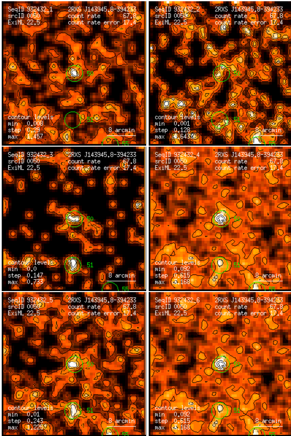
Figure 50: RASS 932432: detection 0050: band rate images, Gaussian filter: (1) PSPC channels 11 – 41, (2) 52 – 90, (3) 91 – 201, (4) 11 – 235, (5) 52 – 201, (6) 11 – 201. Broad band rates in counts/ks. Band rate contour levels in counts/ks/arcmin 2 .
