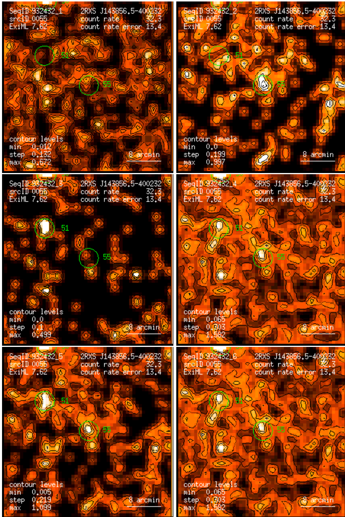
Figure 55: RASS 932432: detection 0055: band rate images, Gaussian filter: (1) PSPC channels 11 – 41, (2) 52 – 90, (3) 91 – 201, (4) 11 – 235, (5) 52 – 201, (6) 11 – 201. Broad band rates in counts/ks. Band rate contour levels in counts/ks/arcmin 2 .
