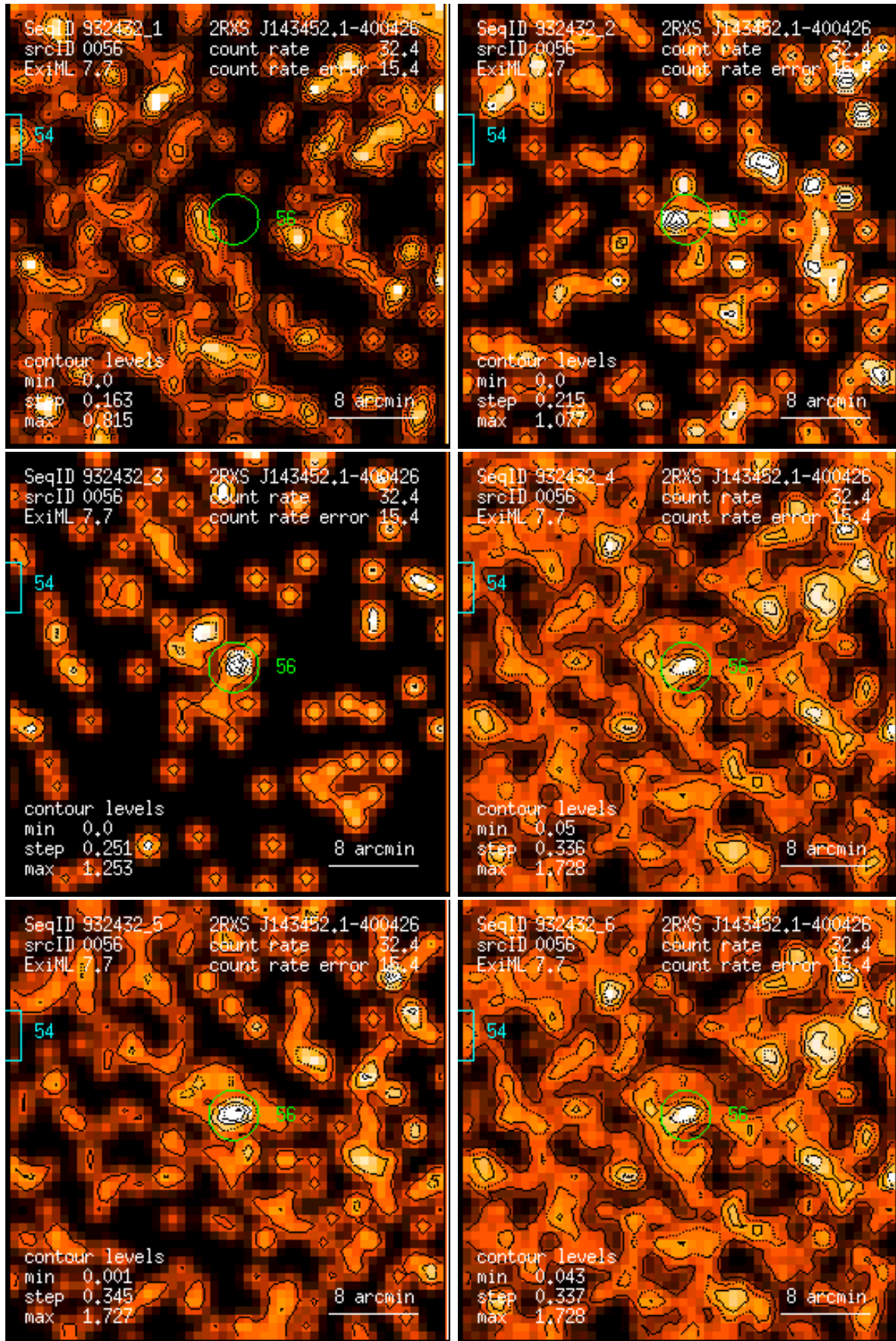
Figure 56: RASS 932432: detection 0056: band rate images, Gaussian filter: (1) PSPC channels 11 – 41, (2) 52 – 90, (3) 91 – 201, (4) 11 – 235, (5) 52 – 201, (6) 11 – 201. Broad band rates in counts/ks. Band rate contour levels in counts/ks/arcmin 2 .
