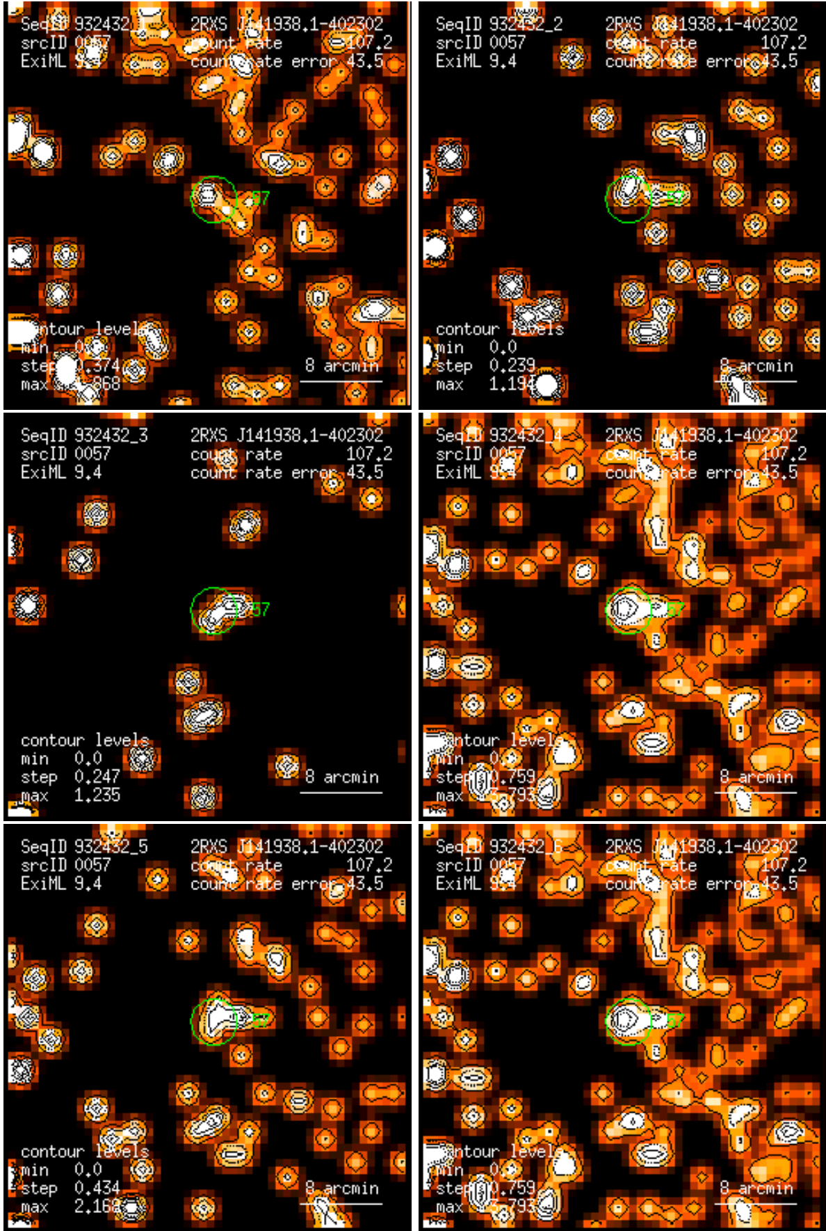
Figure 57: RASS 932432: detection 0057: band rate images, Gaussian filter: (1) PSPC channels 11 – 41, (2) 52 – 90, (3) 91 – 201, (4) 11 – 235, (5) 52 – 201, (6) 11 – 201. Broad band rates in counts/ks. Band rate contour levels in counts/ks/arcmin 2 .
