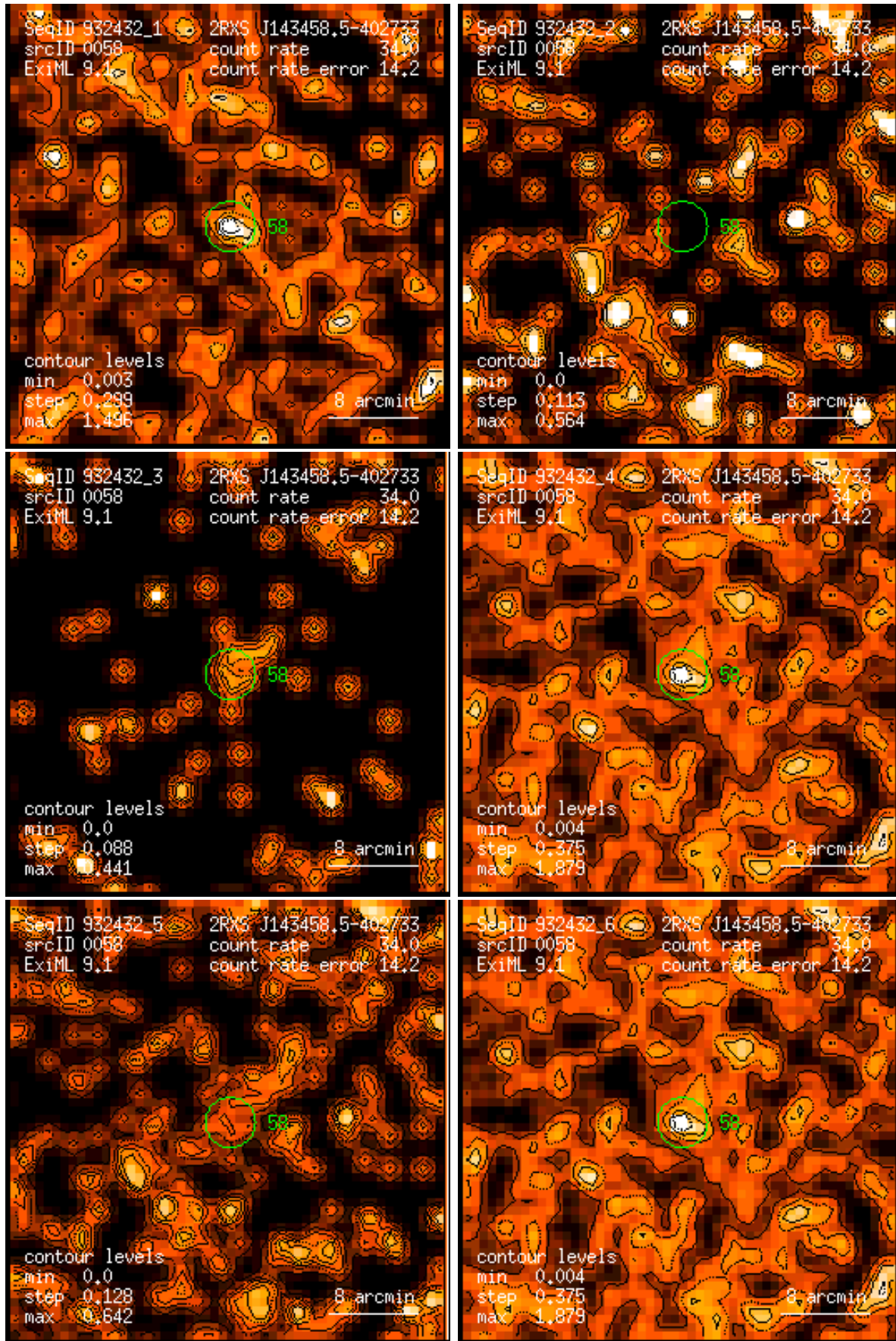
Figure 58: RASS 932432: detection 0058: band rate images, Gaussian filter: (1) PSPC channels 11 – 41, (2) 52 – 90, (3) 91 – 201, (4) 11 – 235, (5) 52 – 201, (6) 11 – 201. Broad band rates in counts/ks. Band rate contour levels in counts/ks/arcmin 2 .
