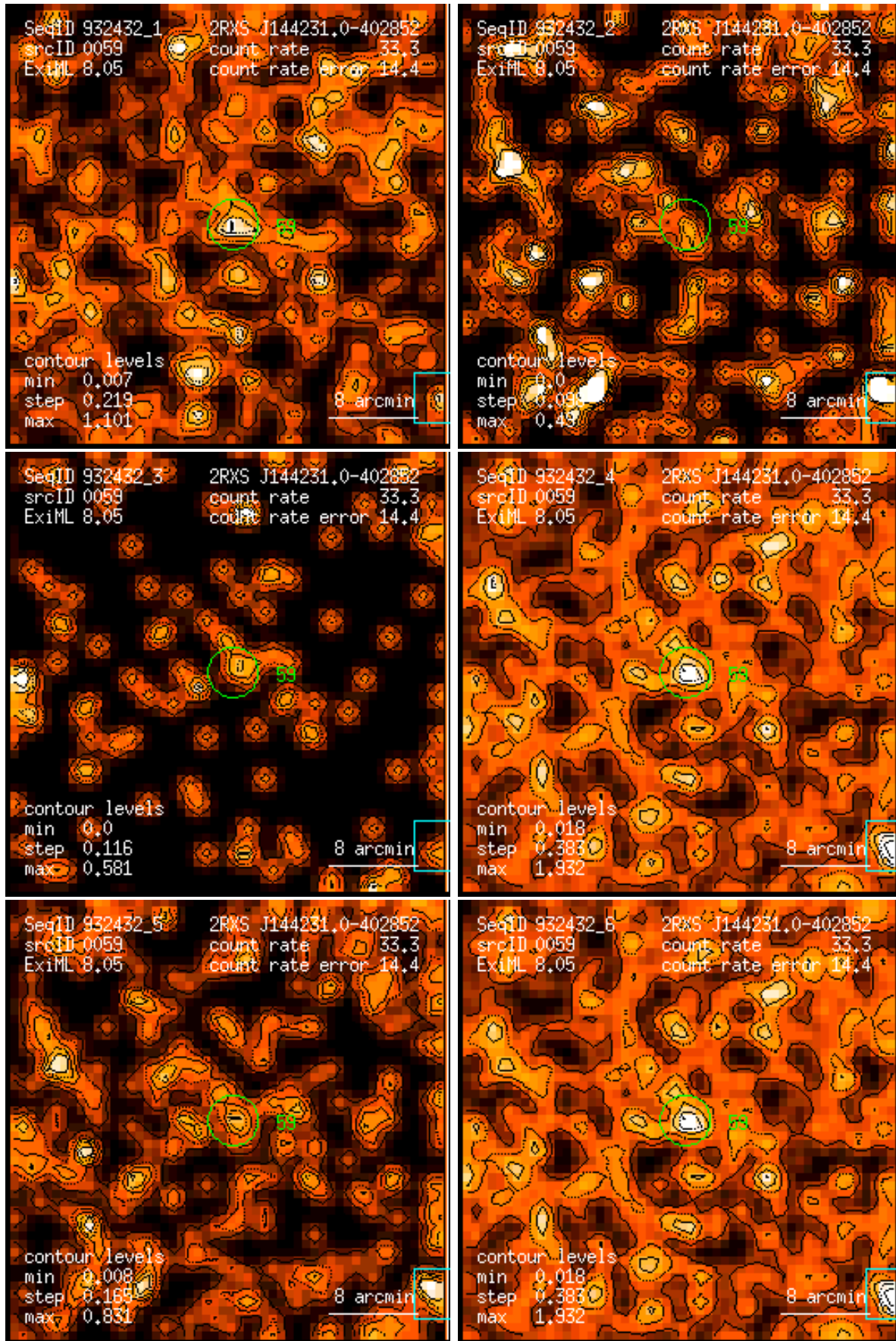
Figure 59: RASS 932432: detection 0059: band rate images, Gaussian filter: (1) PSPC channels 11 – 41, (2) 52 – 90, (3) 91 – 201, (4) 11 – 235, (5) 52 – 201, (6) 11 – 201. Broad band rates in counts/ks. Band rate contour levels in counts/ks/arcmin 2 .
