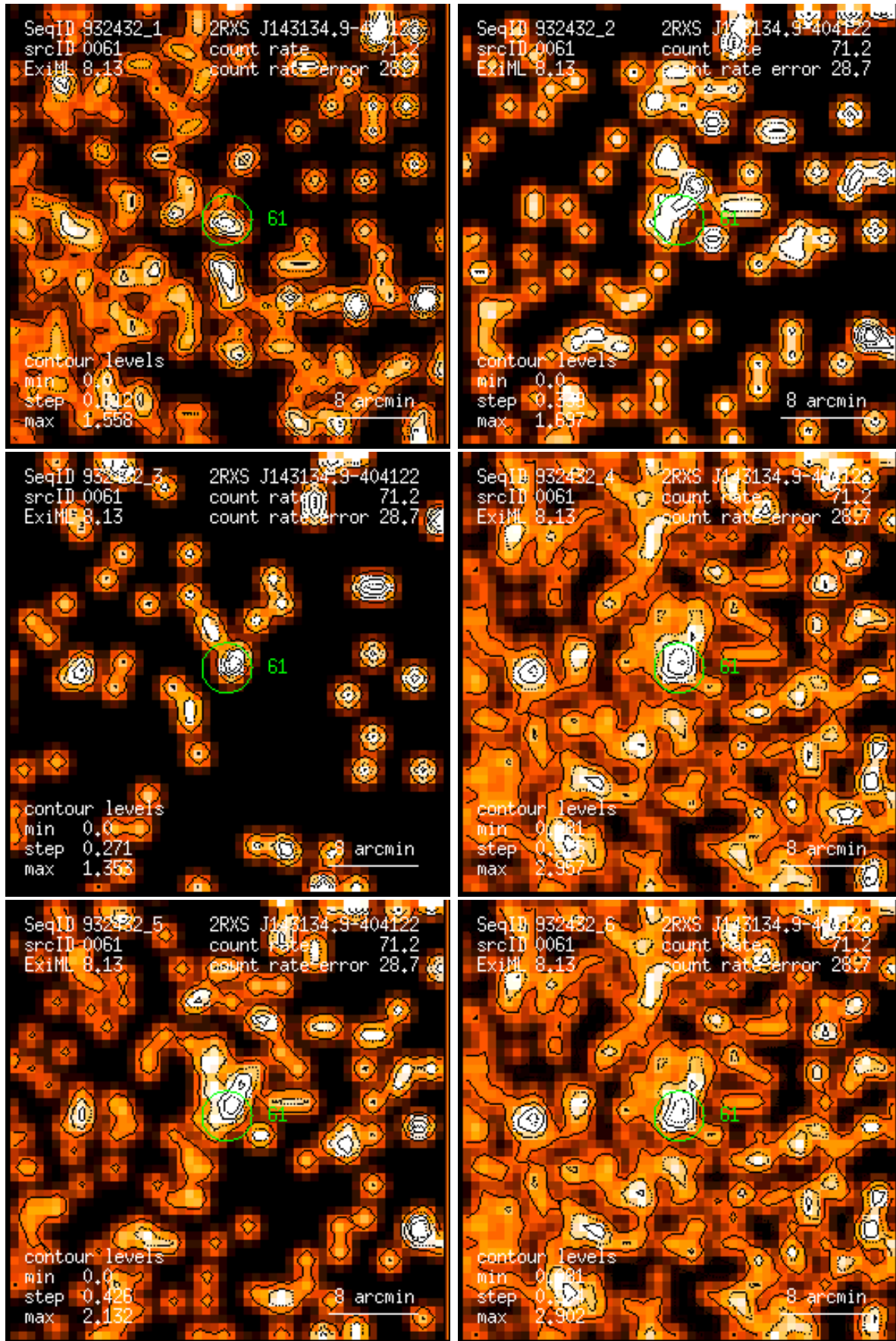
Figure 61: RASS 932432: detection 0061: band rate images, Gaussian filter: (1) PSPC channels 11 – 41, (2) 52 – 90, (3) 91 – 201, (4) 11 – 235, (5) 52 – 201, (6) 11 – 201. Broad band rates in counts/ks. Band rate contour levels in counts/ks/arcmin 2 .
