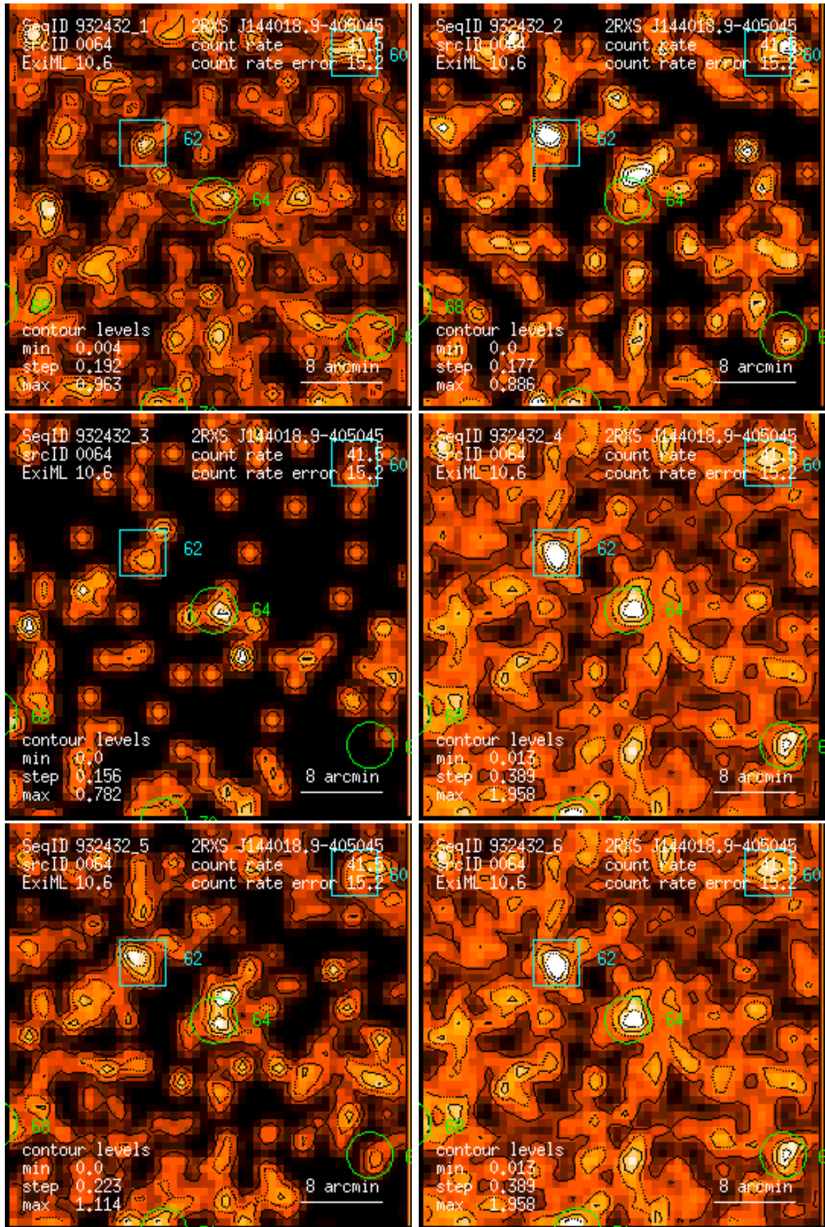
Figure 64: RASS 932432: detection 0064: band rate images, Gaussian filter: (1) PSPC channels 11 – 41, (2) 52 – 90, (3) 91 – 201, (4) 11 – 235, (5) 52 – 201, (6) 11 – 201. Broad band rates in counts/ks. Band rate contour levels in counts/ks/arcmin 2 .
