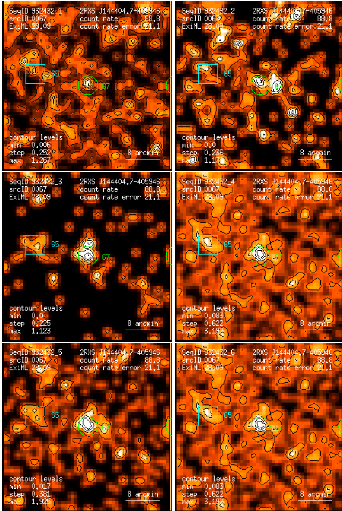
Figure 67: RASS 932432: detection 0067: band rate images, Gaussian filter: (1) PSPC channels 11 – 41, (2) 52 – 90, (3) 91 – 201, (4) 11 – 235, (5) 52 – 201, (6) 11 – 201. Broad band rates in counts/ks. Band rate contour levels in counts/ks/arcmin 2 .
