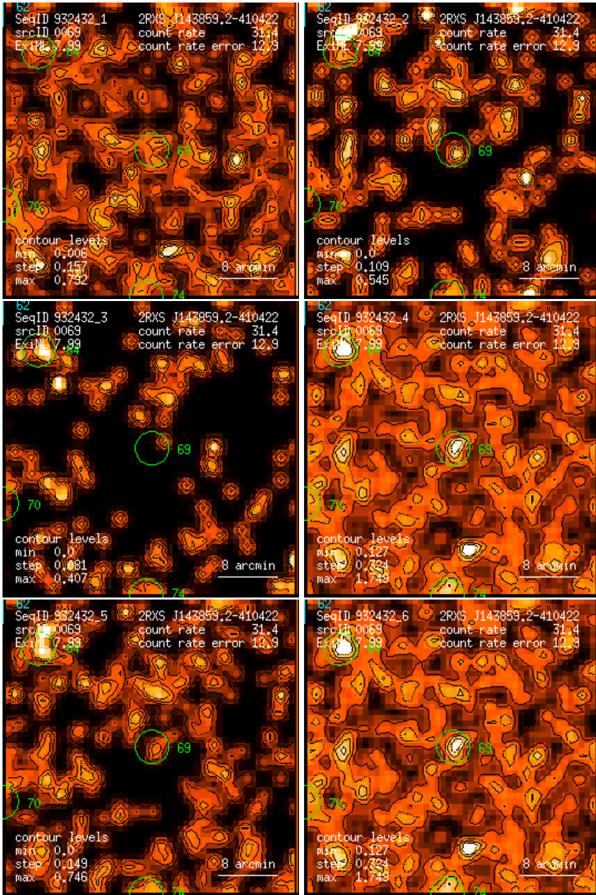
Figure 69: RASS 932432: detection 0069: band rate images, Gaussian filter: (1) PSPC channels 11 – 41, (2) 52 – 90, (3) 91 – 201, (4) 11 – 235, (5) 52 – 201, (6) 11 – 201. Broad band rates in counts/ks. Band rate contour levels in counts/ks/arcmin 2 .
