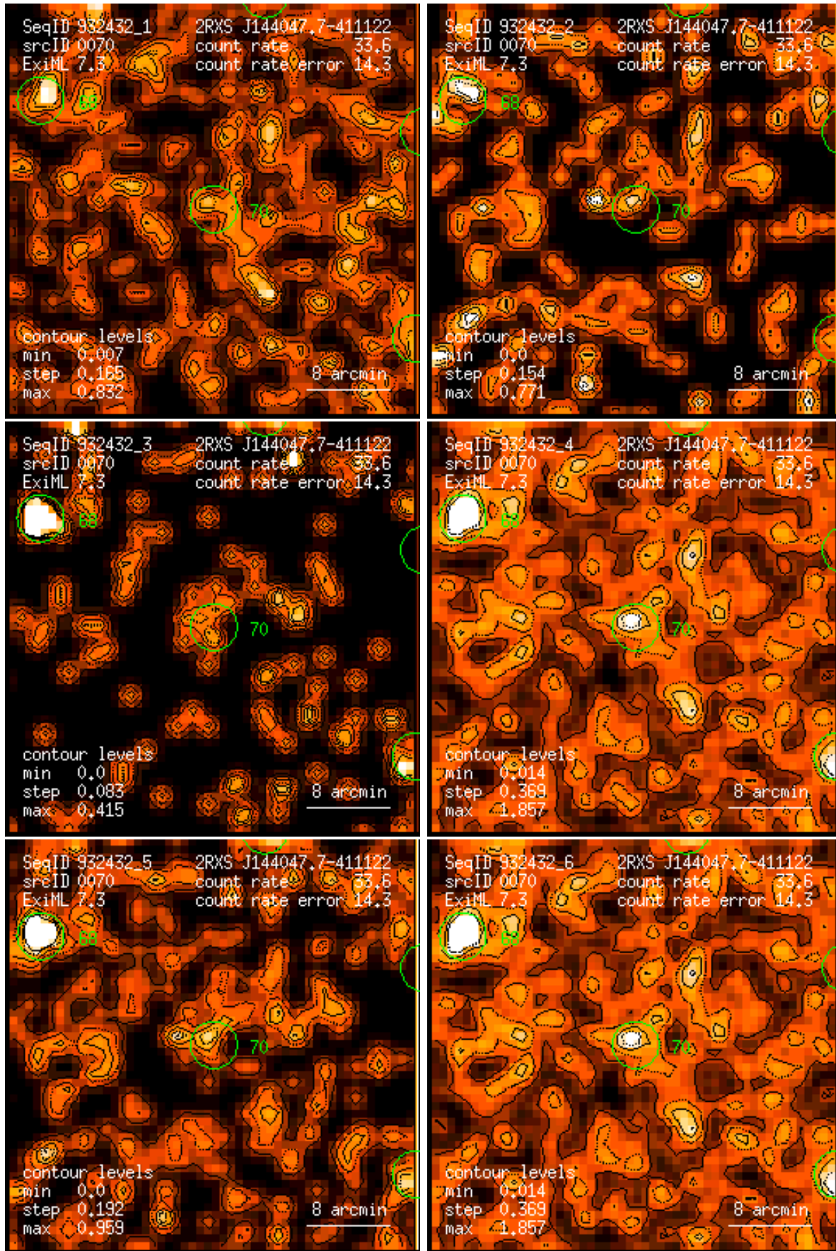
Figure 70: RASS 932432: detection 0070: band rate images, Gaussian filter: (1) PSPC channels 11 – 41, (2) 52 – 90, (3) 91 – 201, (4) 11 – 235, (5) 52 – 201, (6) 11 – 201. Broad band rates in counts/ks. Band rate contour levels in counts/ks/arcmin 2 .
