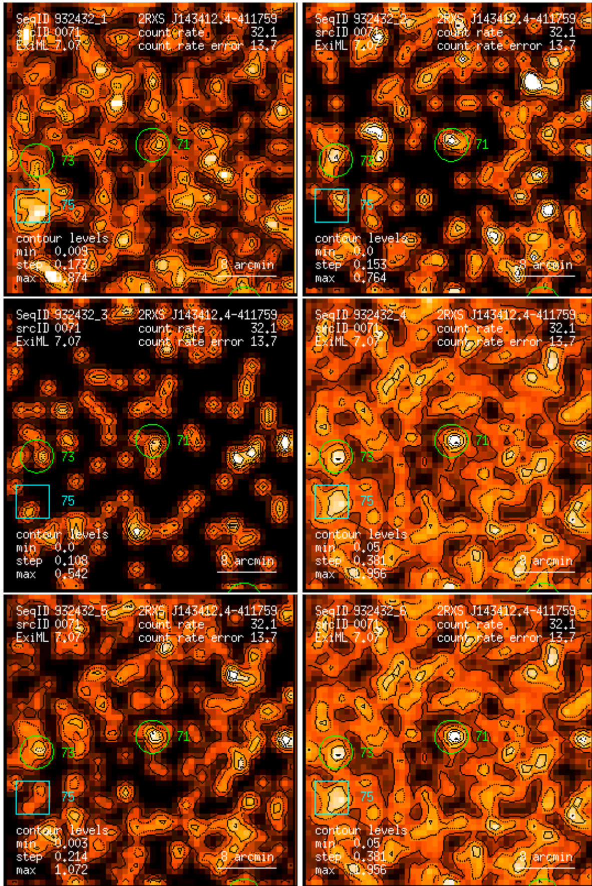
Figure 71: RASS 932432: detection 0071: band rate images, Gaussian filter: (1) PSPC channels 11 – 41, (2) 52 – 90, (3) 91 – 201, (4) 11 – 235, (5) 52 – 201, (6) 11 – 201. Broad band rates in counts/ks. Band rate contour levels in counts/ks/arcmin 2 .
