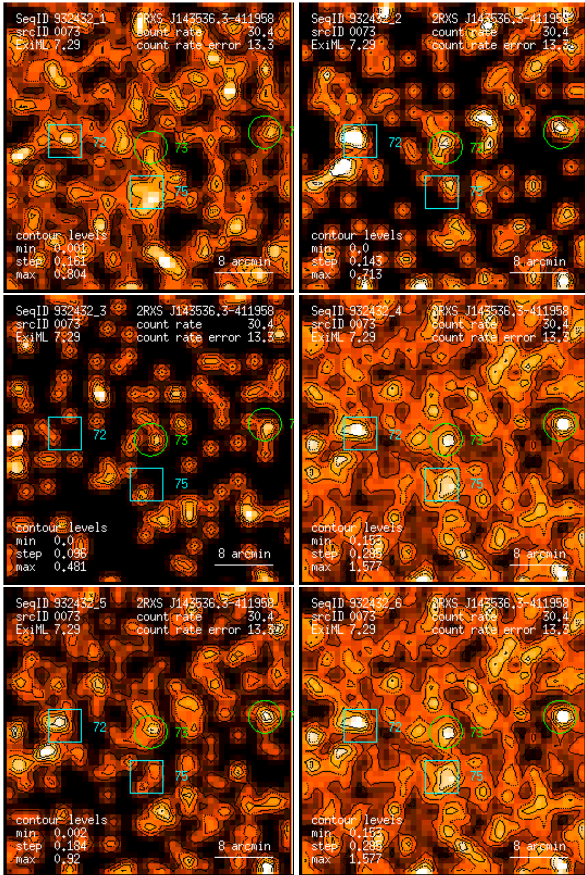
Figure 73: RASS 932432: detection 0073: band rate images, Gaussian filter: (1) PSPC channels 11 – 41, (2) 52 – 90, (3) 91 – 201, (4) 11 – 235, (5) 52 – 201, (6) 11 – 201. Broad band rates in counts/ks. Band rate contour levels in counts/ks/arcmin 2 .
