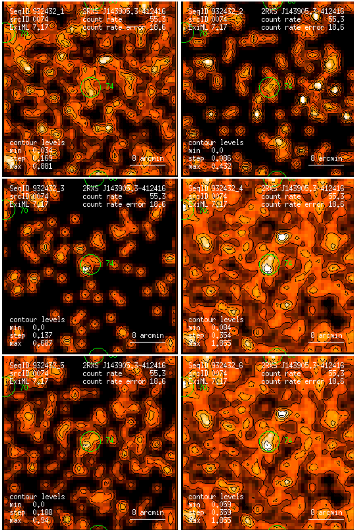
Figure 74: RASS 932432: detection 0074: band rate images, Gaussian filter: (1) PSPC channels 11 – 41, (2) 52 – 90, (3) 91 – 201, (4) 11 – 235, (5) 52 – 201, (6) 11 – 201. Broad band rates in counts/ks. Band rate contour levels in counts/ks/arcmin 2 .
