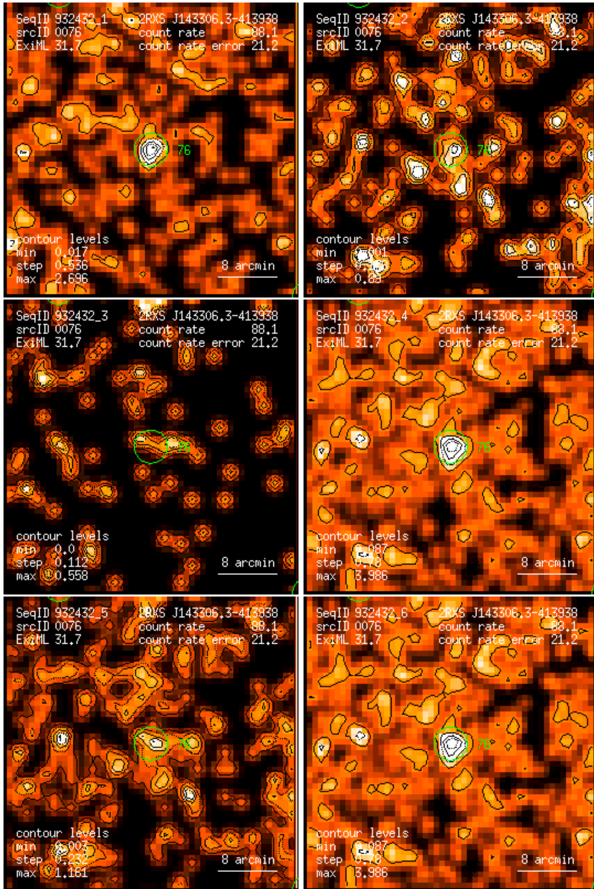
Figure 76: RASS 932432: detection 0076: band rate images, Gaussian filter: (1) PSPC channels 11 – 41, (2) 52 – 90, (3) 91 – 201, (4) 11 – 235, (5) 52 – 201, (6) 11 – 201. Broad band rates in counts/ks. Band rate contour levels in counts/ks/arcmin 2 .
