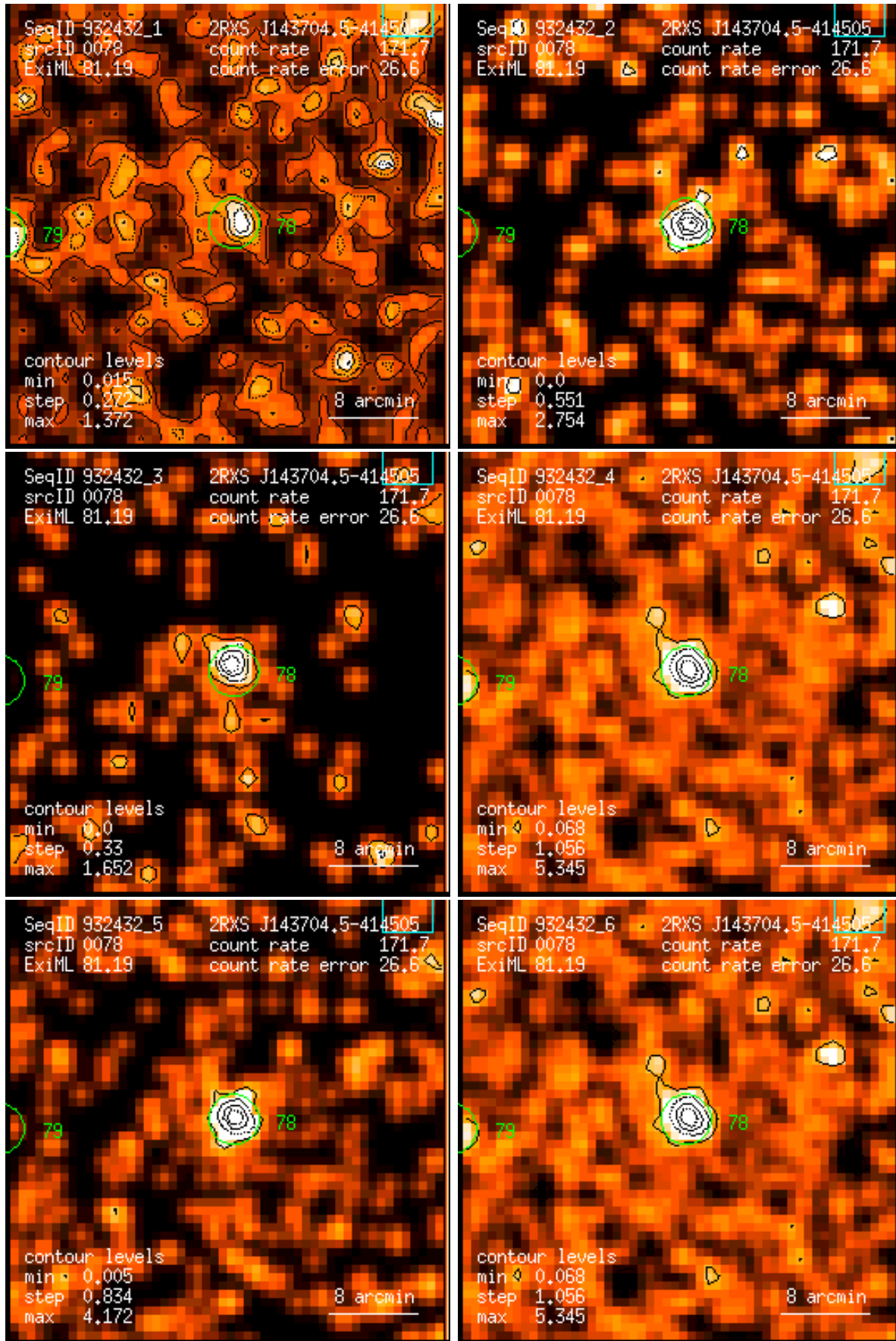
Figure 78: RASS 932432: detection 0078: band rate images, Gaussian filter: (1) PSPC channels 11 – 41, (2) 52 – 90, (3) 91 – 201, (4) 11 – 235, (5) 52 – 201, (6) 11 – 201. Broad band rates in counts/ks. Band rate contour levels in counts/ks/arcmin 2 .
